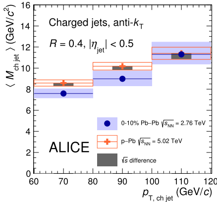
Fig. 9. Fully-corrected mean jet mass as a function of p_{T, \text{ch,jet}} for anti- k_T jets with R = 0.4 in minimum bias p-Pb collisions at \sqrt{s_{NN}} = 5.02 TeV compared to central Pb-Pb collisions at \sqrt{s_{NN}} = 2.76 TeV.
