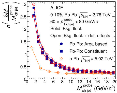
Fig. 3. Jet mass resolution as a function of true jet mass M_{ch\,jet}^{probe} for probes with 60 < p_{T,ch\,jet}^{probe} (GeV/c) < 80 GeV/c. Pb–Pb: Anti- k_T PYTHIA jets with R = 0.4 embedded into central Pb–Pb collisions taking into account background fluctuations and detector effects. p–Pb: 4-vectors corresponding to detector-level PYTHIA jets embedded into p–Pb events.
