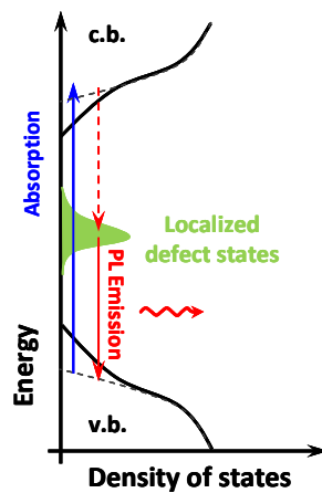
Figure 2.1: Schematic representation of the typical band diagram in semiconductors and intra-band absorption/emission processes.
