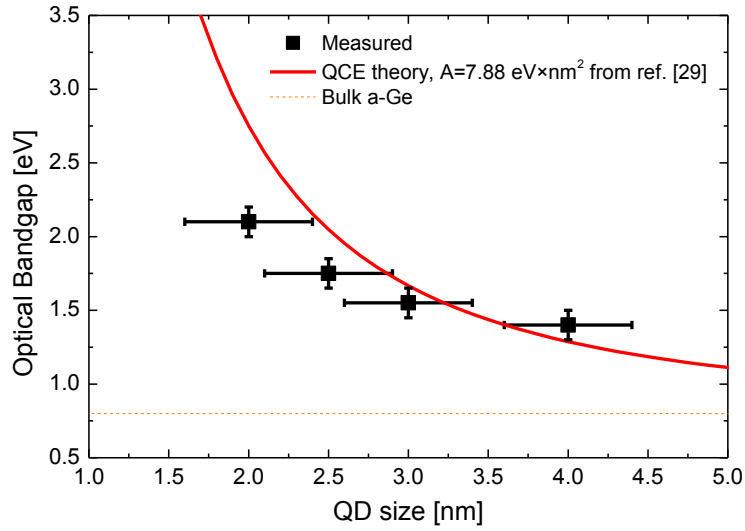
Figure 3.7: Optical bandgap as a function of size for Ge QDs in SiO 2 . The value of amorphous bulk Ge (dashed line) as well as the theoretical trend of E_g for Ge QDs according to ref. [29] are reported for comparison.
