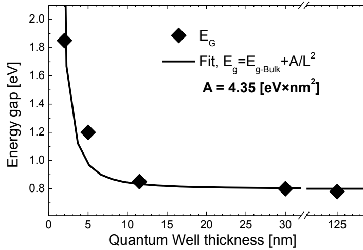
Figure 2.11: Experimental values (diamonds) of energy gap in a-Ge QW versus thickness, fitted through effective mass theory formula of QC (Eq. (1.4), solid line). Adapted from ref. [83].
