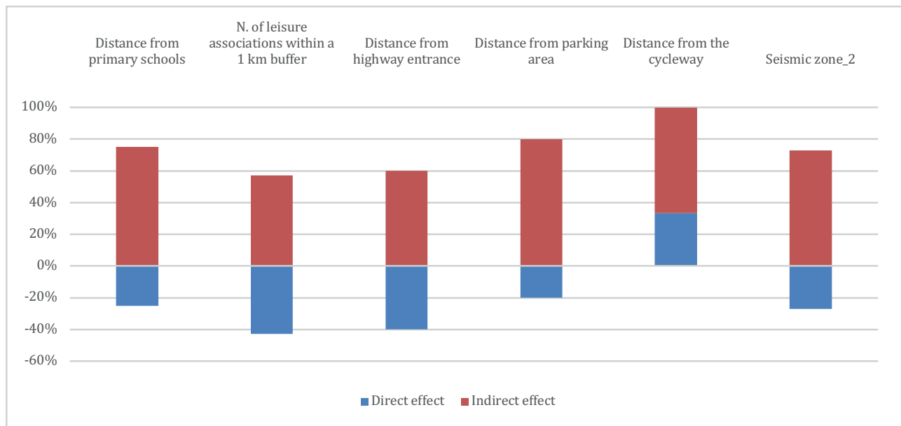
Figure 3. Total, direct and indirect effects.
