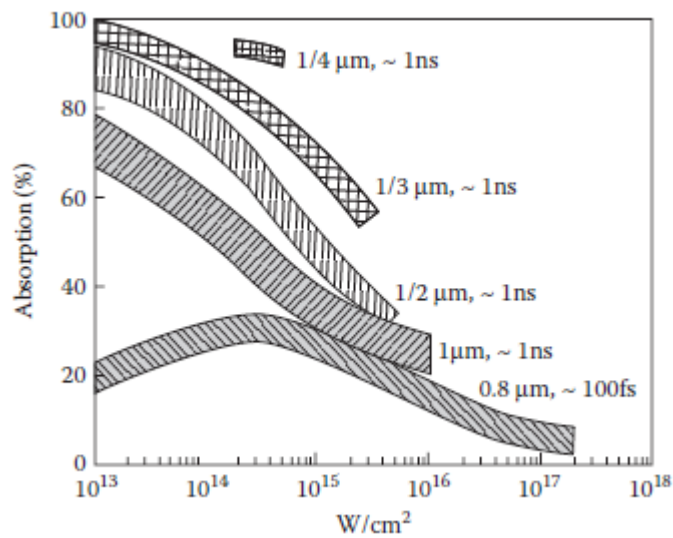
Fig. 1.3.1 – Experimental data of the laser absorption in solid low-Z targets [19].
