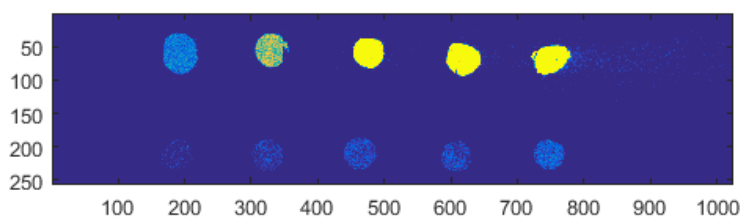
Fig. 4.2.1 – X-ray images of a plasma obtained simultaneously from a single shot by using a 10-channel pinhole-camera, where each channel indicates a different spectral region.
