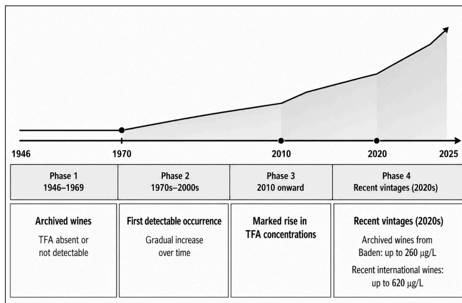
Figure 1. Historical evolution of TFA occurrence in wine based on archived-wine evidence.
