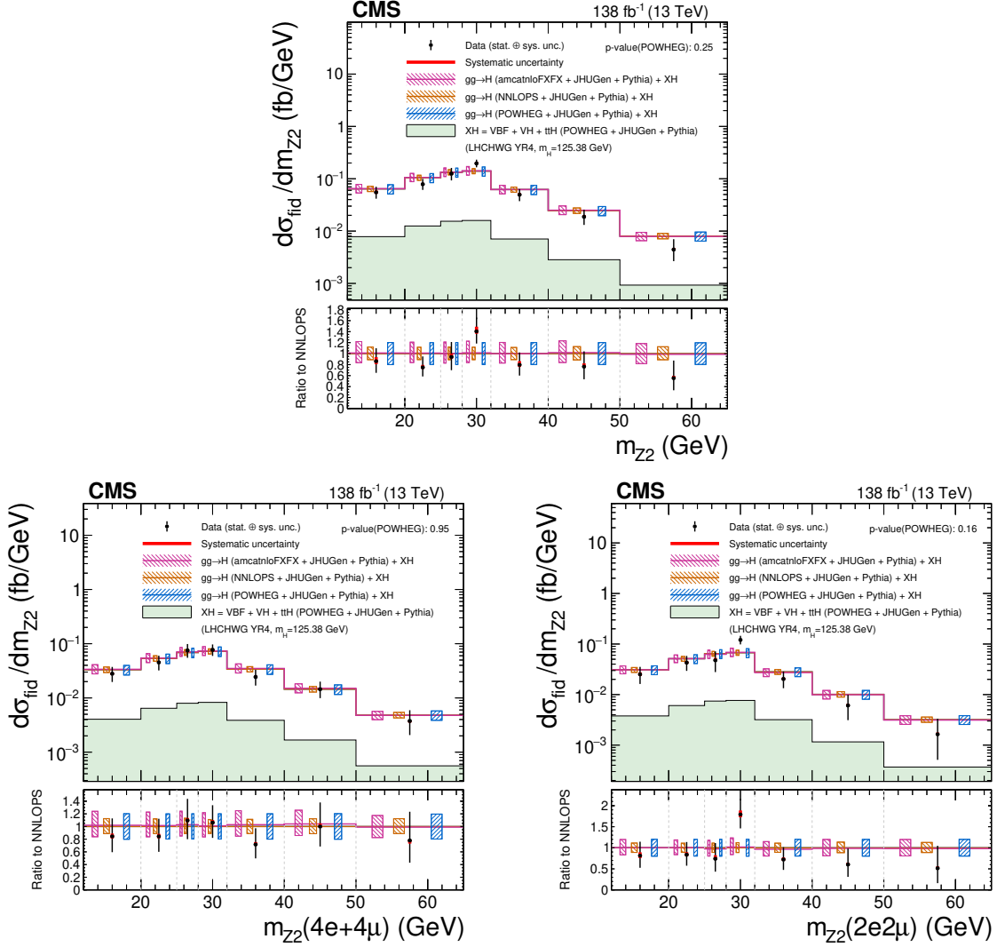
Figure 12. Differential cross sections as functions of the invariant mass of the subleading dilepton pair m_{Z_2} in the 4 \ell (upper) and in the same-flavor (lower left) and different-flavor (lower right) final states. The acceptance and theoretical uncertainties in the differential bins are calculated using the ggH predictions from three different generators normalized to next-to-next-to-next-to-leading order (N 3 LO) [34]. The subdominant component of the signal (VBF + VH + ttH) is denoted as XH and is fixed to the SM prediction. The measured cross sections are compared with the ggH predictions from POWHEG (blue), NNLOPS (orange), and MADGRAPH5_AMC@NLO (pink). The hatched areas correspond to the systematic uncertainties in the theoretical predictions. Black points represent the measured fiducial cross sections in each bin, black error bars the total uncertainty in each measurement, red boxes the systematic uncertainties. The lower panels display the ratios of the measured cross sections and of the predictions from POWHEG and MADGRAPH5_AMC@NLO to the NNLOPS theoretical predictions.
