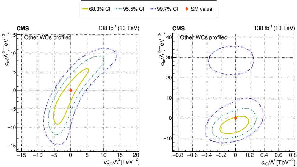
Figure 10. The observed 68.3, 95.5, and 99.7% confidence level contours of a 2D scan with the other WCs profiled, for c_{\varphi Q} and c_{\varphi t} (left), and for c_{tG} and c_{t\varphi} (right). Diamond markers show the SM prediction.
