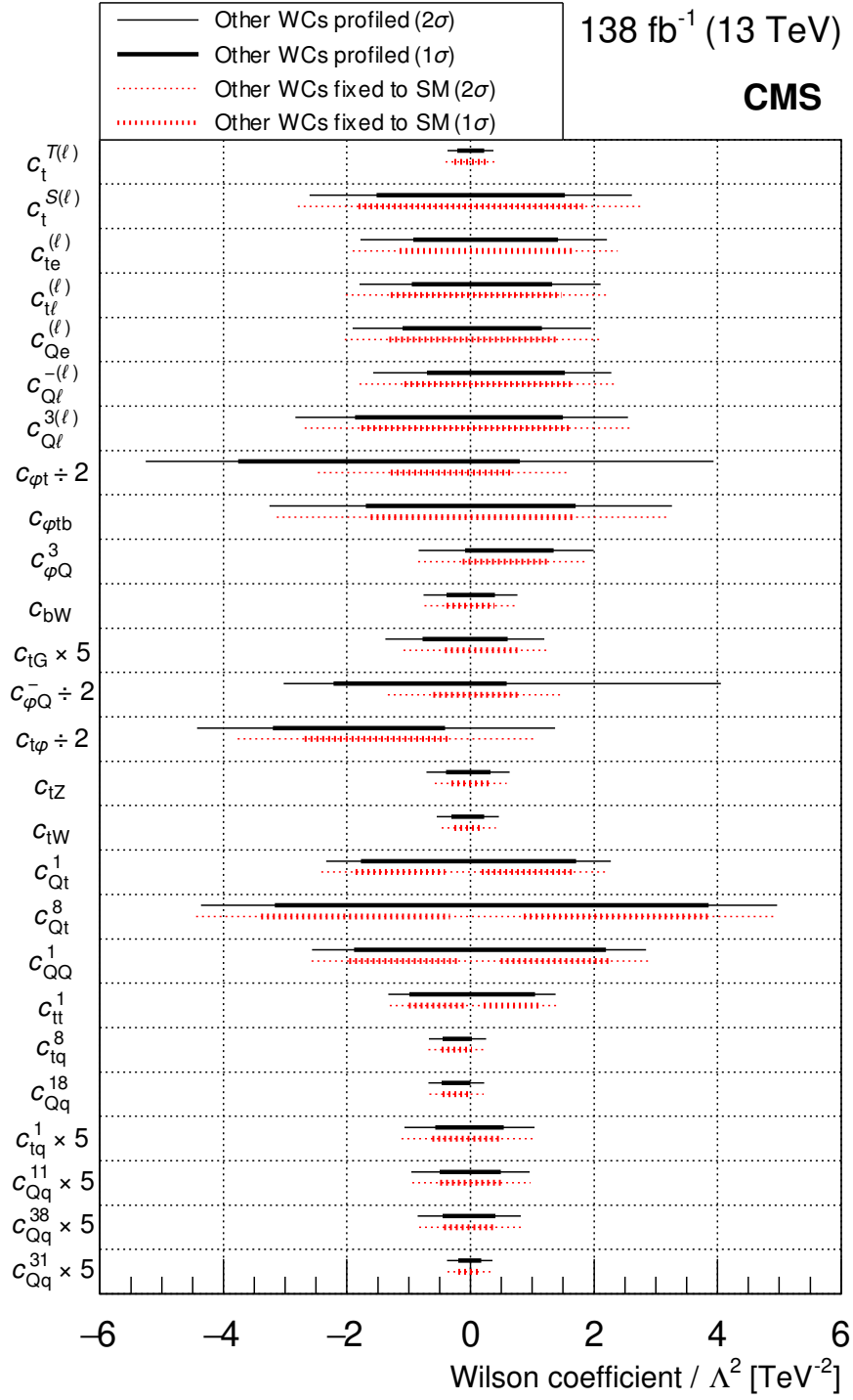
Figure 8. Summary of CIs extracted from the likelihood fits described in section 7. The WC 1σ (thick line) and 2σ (thin line) CIs are shown for the case where the other WCs are profiled (in solid black), and the case where the other WCs are fixed to their SM values of zero (in dashed red). To make the figure more readable, the intervals for c_{t\phi} , c_{\phi t} , and c_{\phi Q}^- were scaled by 0.5, and the intervals for c_{tG} , c_{tq}^1 , c_{Qq}^{11} , c_{Qq}^{38} , and c_{Qq}^{31} were scaled by 5.
