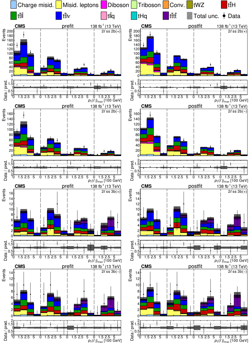
Figure 4. The categories shown in these plots are 2\ell ss\ 2b and 2\ell ss\ 3b . The prefit plots for each category are shown on the left side while the postfit plots are shown on the right side. The differential distribution in the plots is p_T(\ell j)_{\max} . The jet subcategories are arranged from low jet multiplicity to high jet multiplicity from left to right for each individual plot. For example, in the 2\ell ss\ 2b\ (+) plot, the first four bins are the p_T(\ell j)_{\max} variable for 2\ell ss\ 2b\ (+)\ 4j , the next four bins are for 2\ell ss\ 2b\ (+)\ 5j , etc. The process labeled “Conv.” corresponds to the photon conversion background, “Misid. leptons” corresponds to misidentified leptons, and “Charge misid.” corresponds to leptons with a mismeasured charge.
