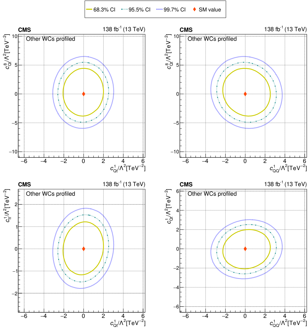
Figure 11. The observed 68.3, 95.5, and 99.7% confidence level contours of a 2D scan with the other WCs profiled, for c_{Q_t}^1 and c_{Q_t}^8 (upper left), for c_{Q_Q}^1 and c_{Q_t}^8 (upper right), for c_{Q_t}^1 and c_{t t}^1 (lower left), and for c_{Q_Q}^1 and c_{Q_t}^1 (lower right). Diamond markers show the SM prediction.
