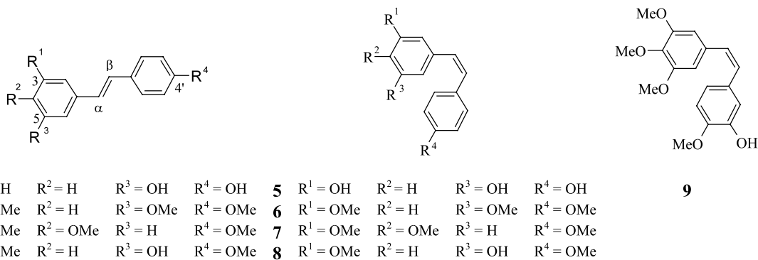
Fig. 1. Structures of compounds 1 – 9 : E -3,5,4'-trihydroxystilbene ( 1 ), E -3,5,4'-trimethoxystilbene ( 2 ), E -3,4,4'-trimethoxystilbene ( 3 ), E -3,4'-dimethoxy-5-hydroxystilbene ( 4 ), Z -3,5,4'-trihydroxystilbene ( 5 ), Z -3,5,4'-trimethoxystilbene ( 6 ), Z -3,4,4'-trimethoxystilbene ( 7 ), Z -3,4'-dimethoxy-5-hydroxystilbene ( 8 ) and combretastatin A-4 ( 9 ).
