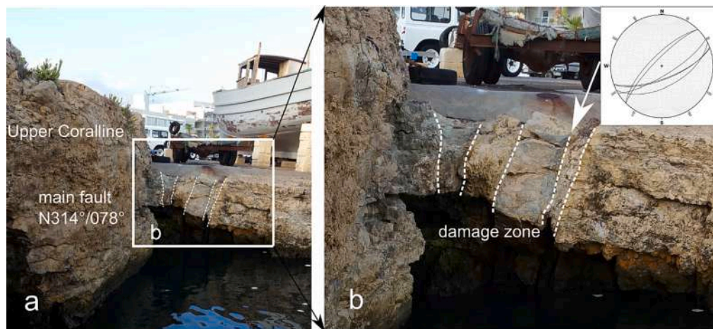
Fig. 6. Evidence of the NE termination of the fault bounding the Mellieha bay to the south-east. (a) NW-dipping normal fault zone ( N314^{\circ}/078^{\circ} ) affecting the Upper Coralline Fm. at the Mellieha Harbor (Dawret it-Tunara, coordinates E14.356949^{\circ} , N35.966816^{\circ} ). (b) Detail of the small-displacement fault damage zone. Fault attitude notation is dip direction/dip angle.
