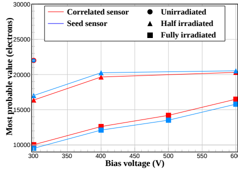
Figure 30. Most probable value of the Landau distribution as a function of the bias voltage for different irradiation fluences.
