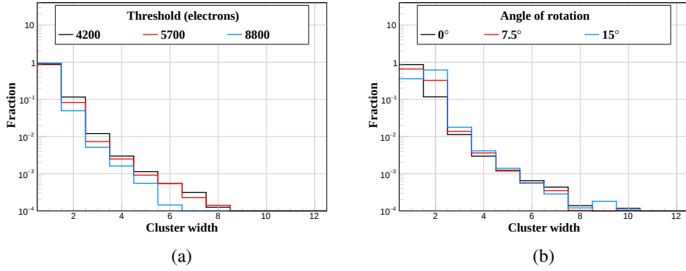
Figure 21. Cluster width for selected values of V_{CTH} (a) and incident angle (b) for the unirradiated mini-module.
