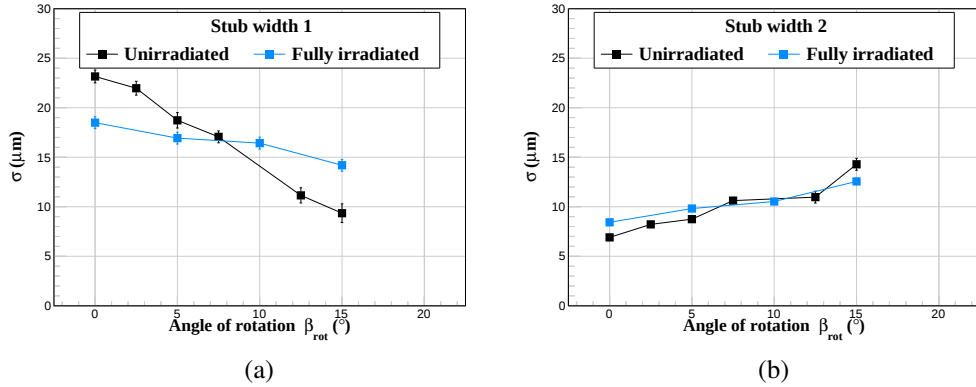
Figure 27. Stub resolution as a function of incident angle for clusters of width one (a) and width two (b). Results are shown for the stubs of the unirradiated and fully irradiated mini-module.
