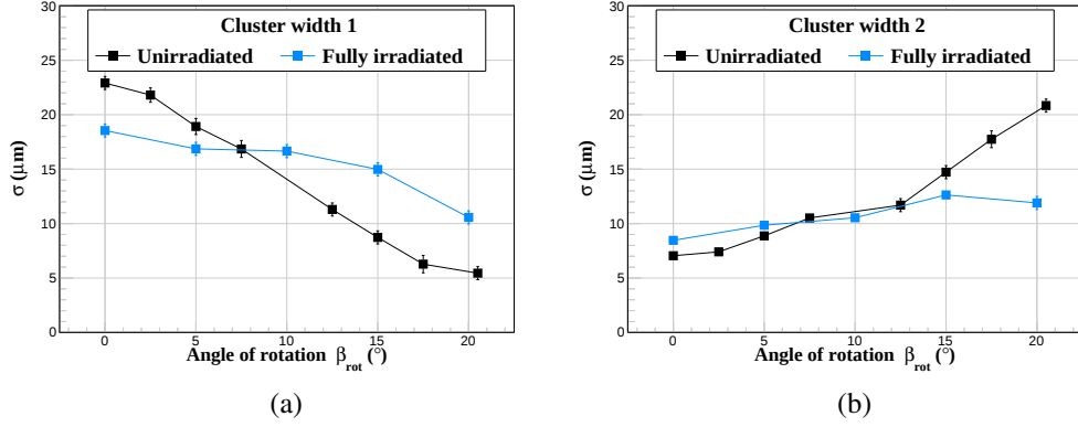
Figure 26. Resolution as a function of incident angle for clusters of width one (a) and width two (b). Results are shown for the correlated sensor of the unirradiated and fully irradiated mini-module.
