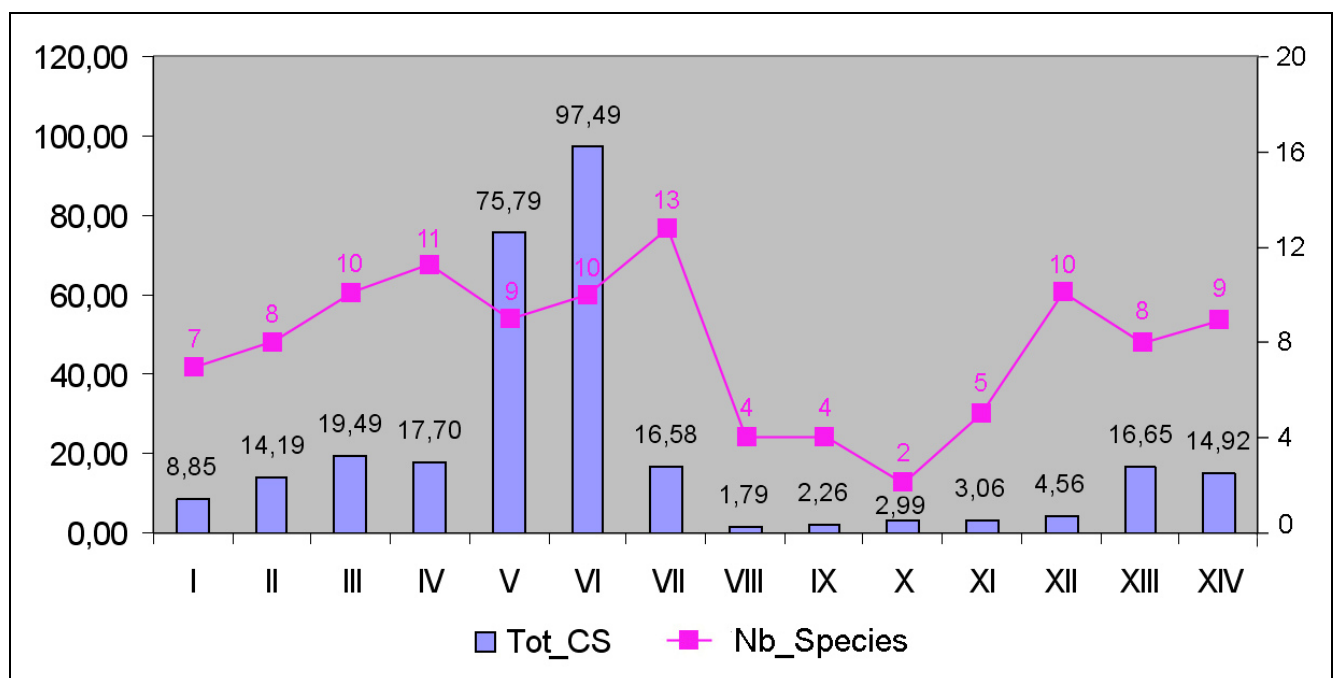
Graph. 5.1.2 - Trends in capture frequencies (CS) of the Coleoptera Carabidae in individual sampling periods and sampled species number.
