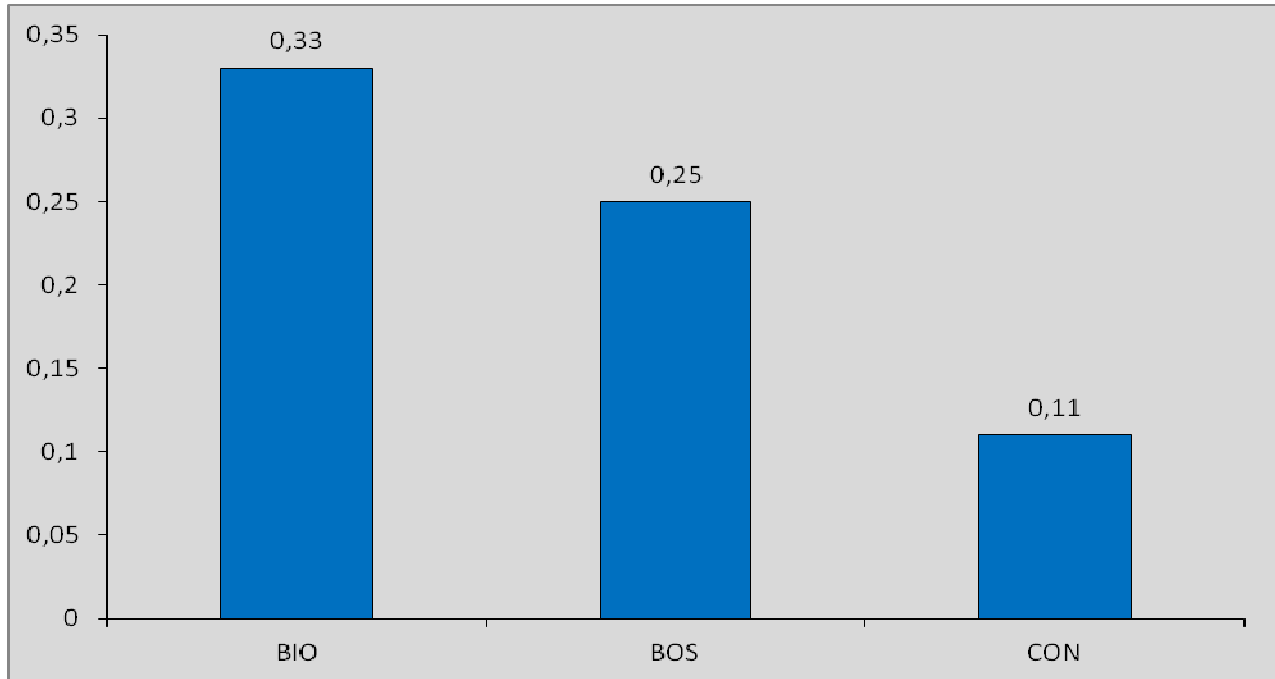
Graph. 5.3.15 - Trend of capture frequency (CS) of Omalium rugatum within the single station.
