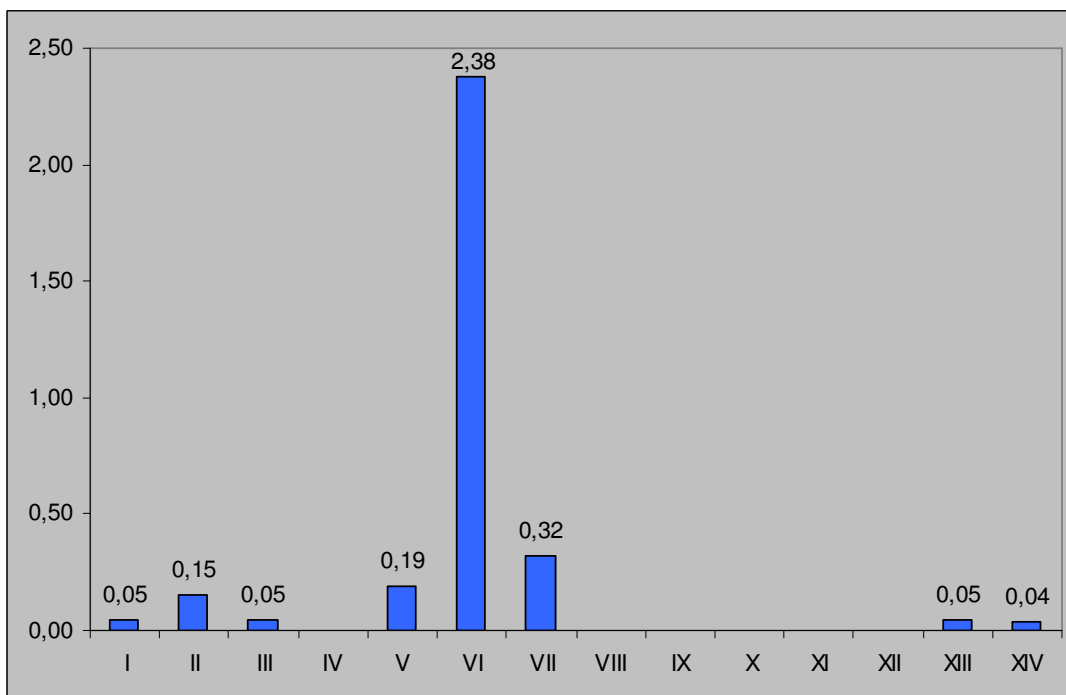
Graph. 5.1.12 - Trends in capture frequencies (CS) of Calathus (Neocalathus) ambiguus in individual sampling periods.
