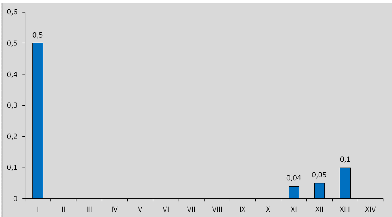
Graph. 5.3.16 - Trends in capture frequencies (CS) of Omalium rugatum in individual sampling periods.
