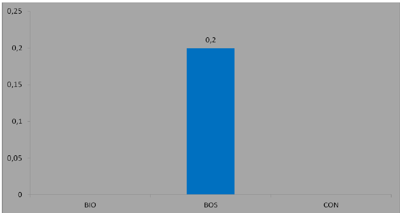
Graph. 5.3.23 - Trend of capture frequency (CS) of Lordithon exoletus within the single station.
