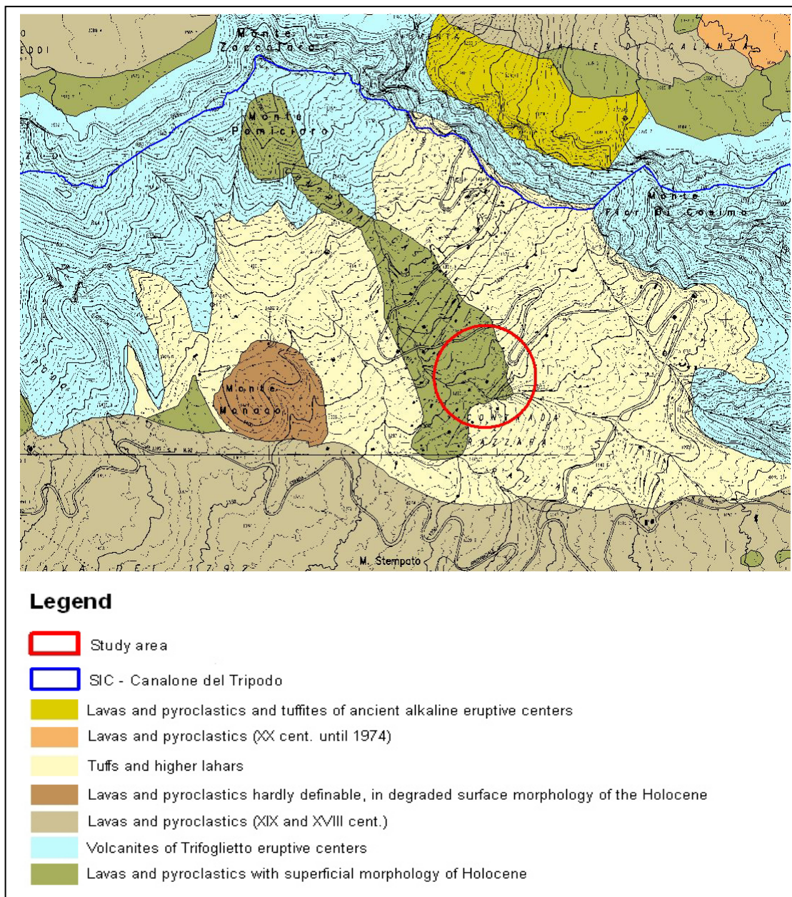
Fig. 2.3.1 - Main geological and geomorphological characteristics of the study area (from draft of Regional Landscape Plan, field 13). The sampling area is shown with a red circle.
