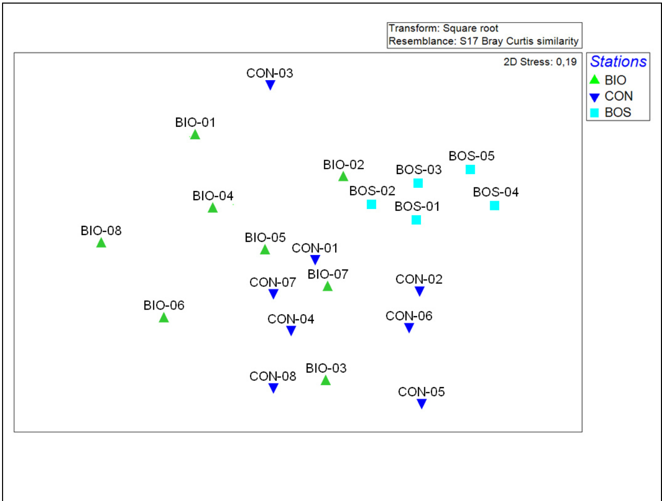
Graph. 7.1.20 – The Nonmetric Multi Dimensional Scaling (NMDS), elaborated on the Bray-Curtis similarity matrix between the traps of investigated stations, in regards to the Staphylinidae species (2 D vision).
