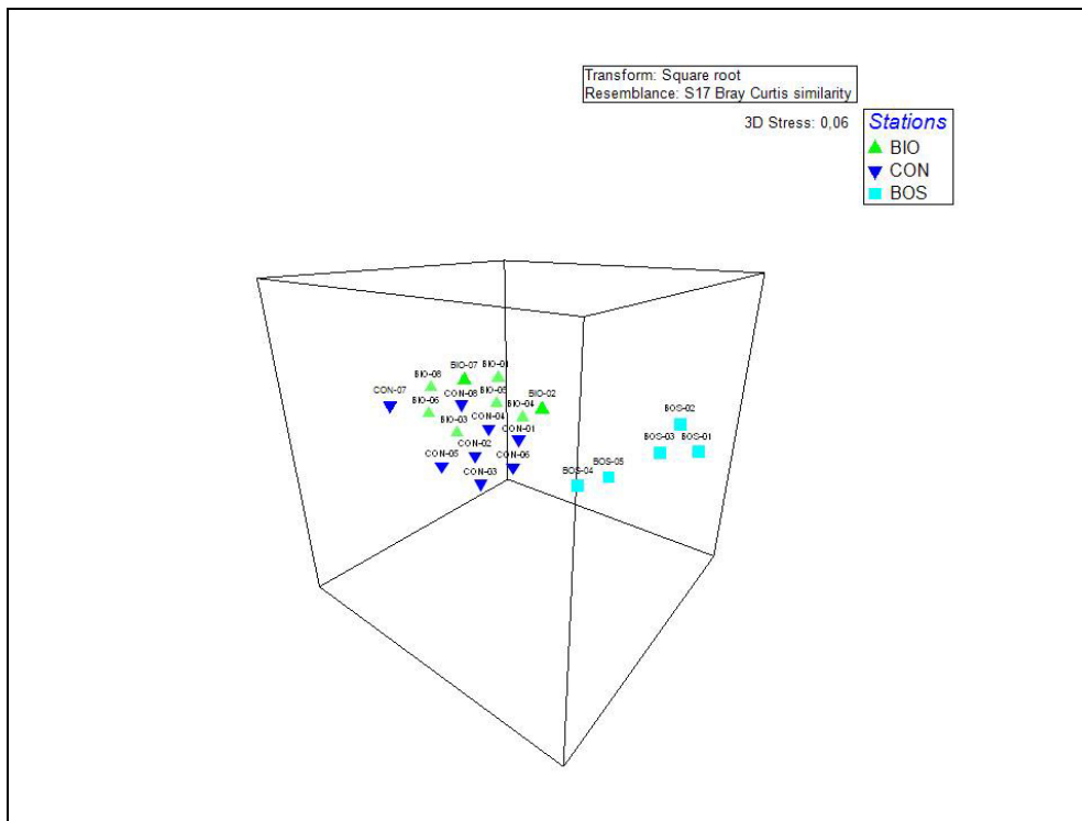
Graph. 7.1.9 – The Nonmetric Multi Dimensional Scaling (NMDS) elaborated on the Bray-Curtis similarity matrix between the traps of investigated stations in regards to Carabidae species (3 D vision).
