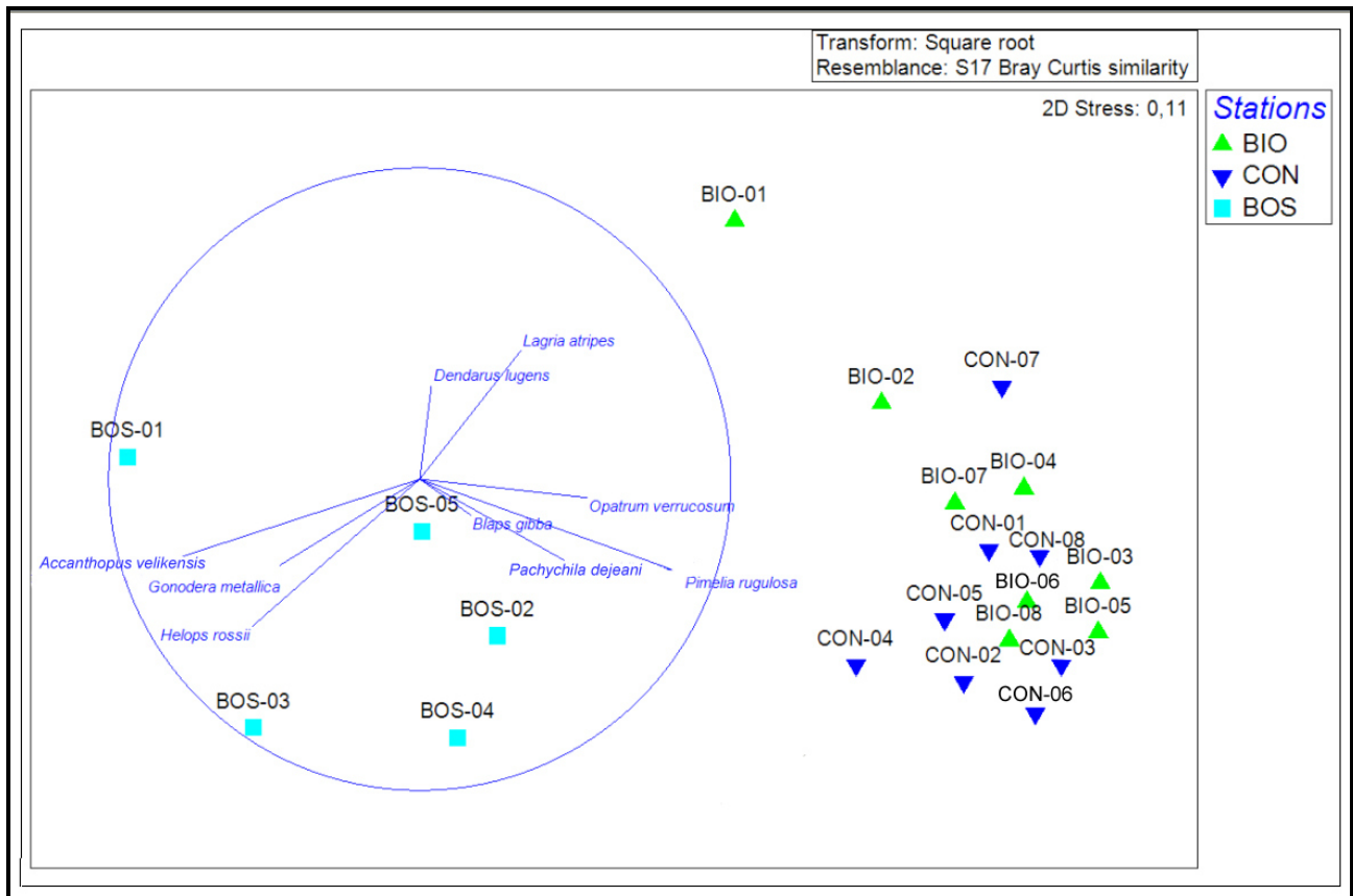
Graph. 7.1.18 – The correlation between Nonmetric Multi Dimensional Scaling (N-MDS) developed on the Bray-Curtis similarity matrix between the stations and the Tenebrionidae species; in the figure only those most abundantly sampled determine the differences or similarities among the traps of three stations are indicated.
