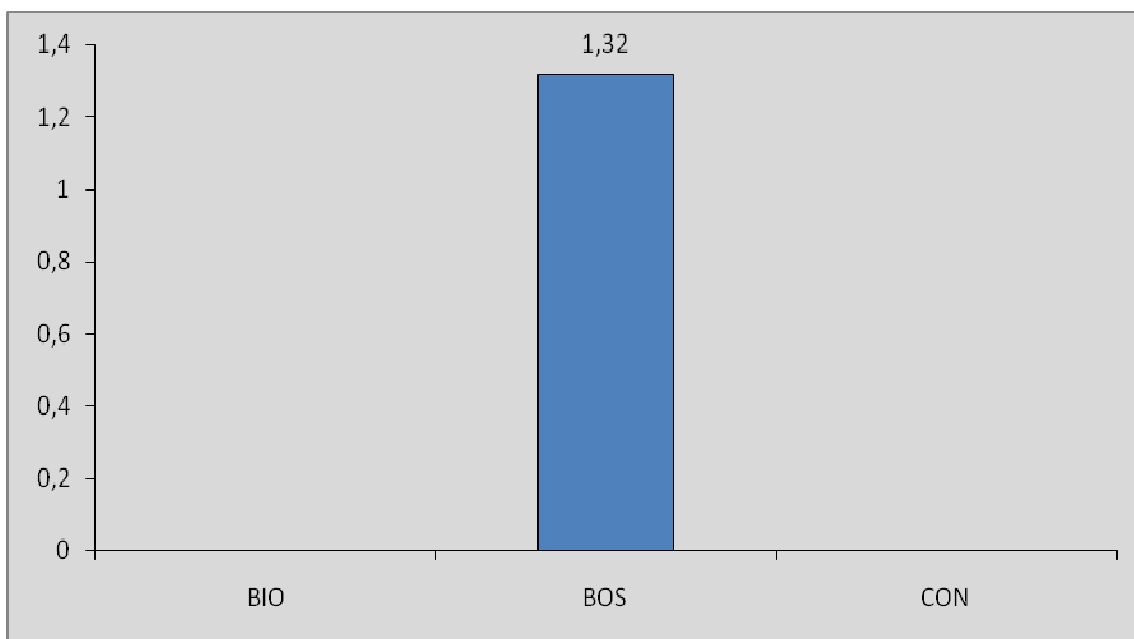
Graph. 5.2.7 - Trend of capture frequency (CS) of Accanthopus velikensis within the single station.
