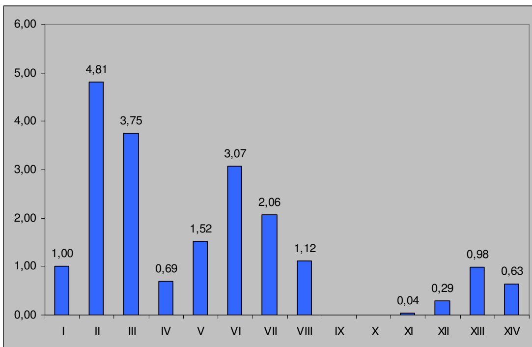
Graph. 5.1.8 - Trends in capture frequencies (CS) of Laemostenus (Pristonychus) algerinus algerinus in individual sampling periods.
