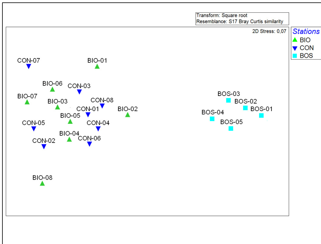
Graph. 7.1.2 - The Nonmetric Multi Dimensional Scaling (NMDS) elaborated on the Bray-Curtis similarity matrix between the traps of investigated stations in regards to Families of the Coleoptera (2 D vision).
