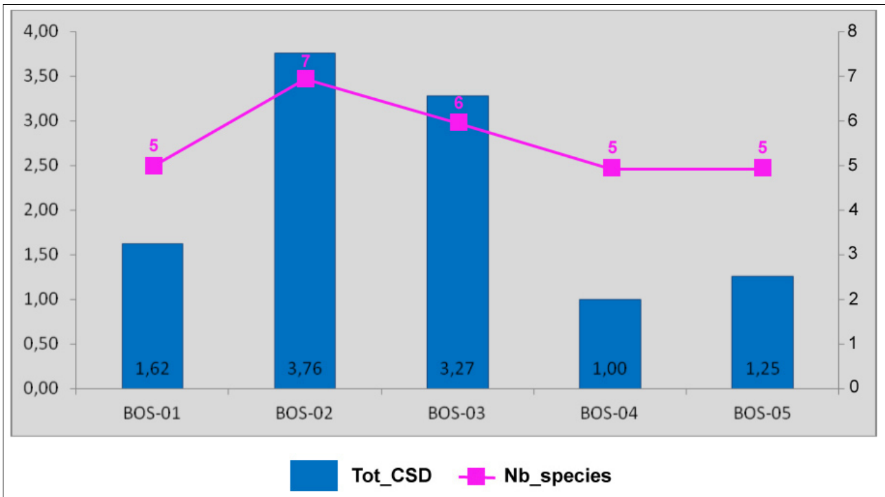
Graph. 6.3.4 - Captures frequency (CS) and Staphylinidae species number in the BOS station traps.
