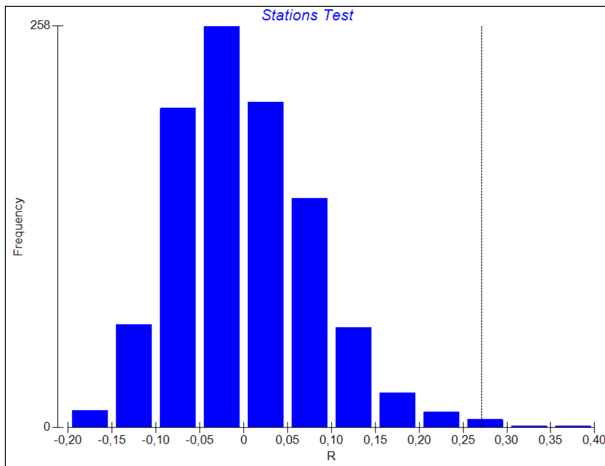
Graph. 7.1.22 – ANOSIM tests: distribution of expected frequencies of R (histogram) compared with the observed value of R (0,27) (continuous line) between the traps of the stations investigated in regards to the Staphylinidae species.
