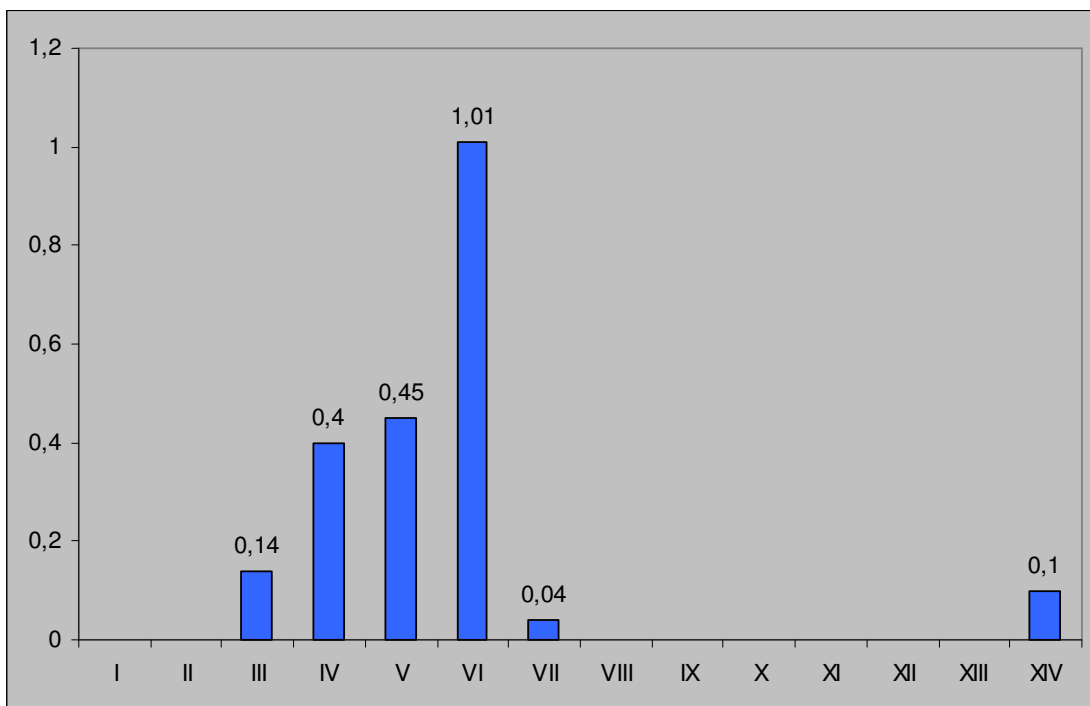
Graph. 5.1.18 - Trends in capture frequencies (CS) of Synuchus vivalis in individual sampling periods.
