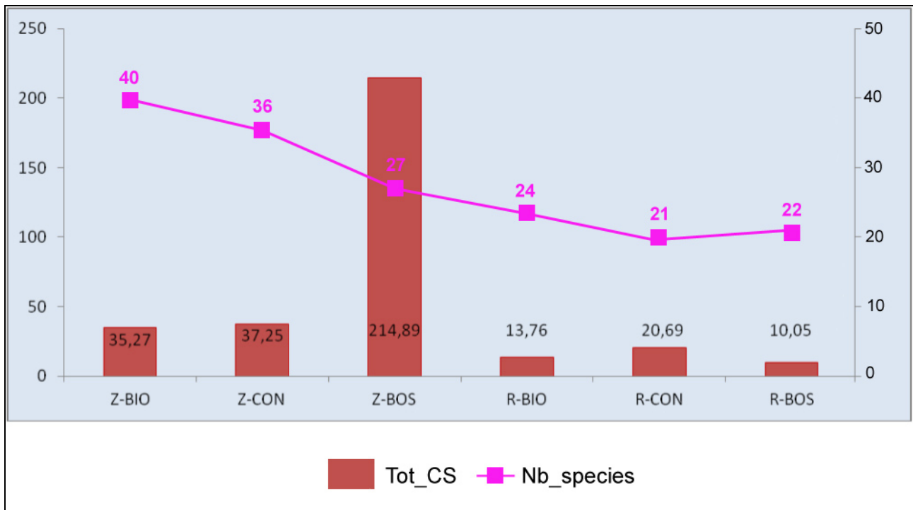
Graph. 8.3.8 - Overall trend of the specimens catches (Tot_CS) and species number (Nb_Species) sampled in each station.
