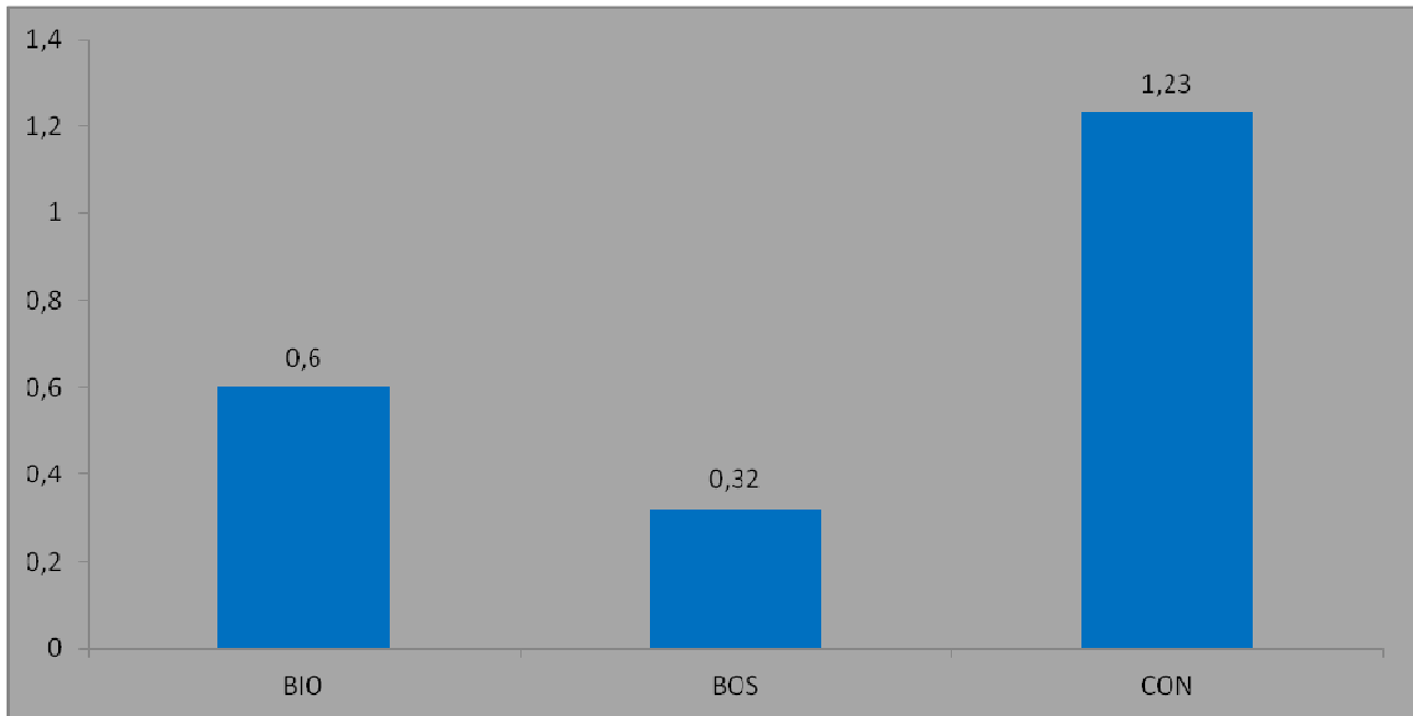
Graph. 5.3.7 - Trend of capture frequency (CS) of Paraphloeostiba gayndahensis within the single station.
