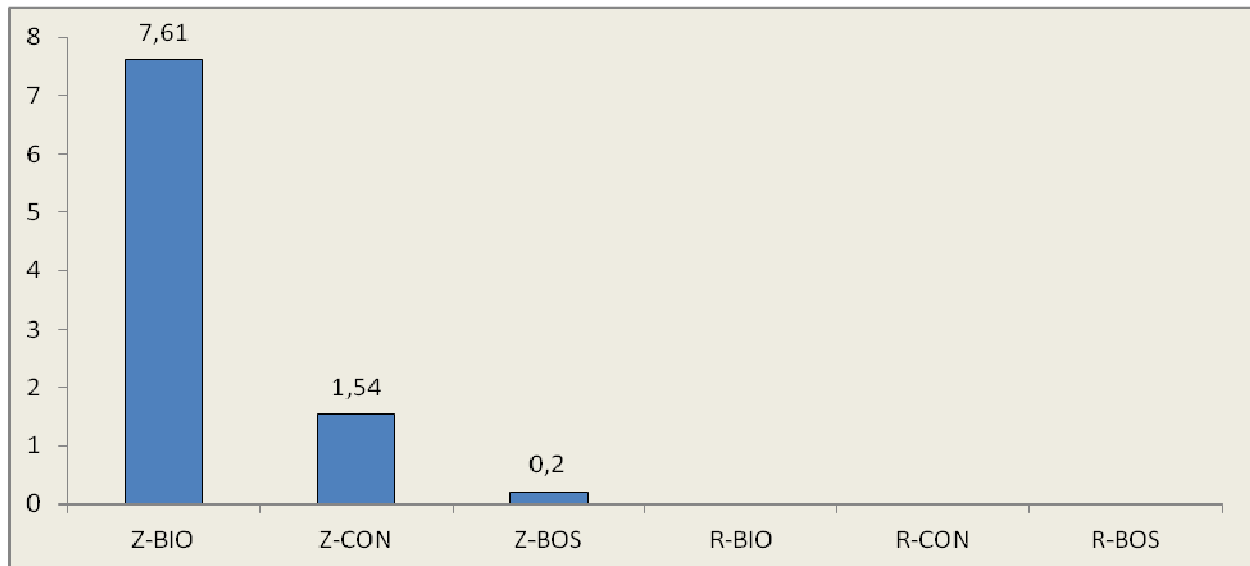
Graph. 8.3.14 - Trend of Synthomus obscuroputtatus captures frequency (CS) within the single station.
