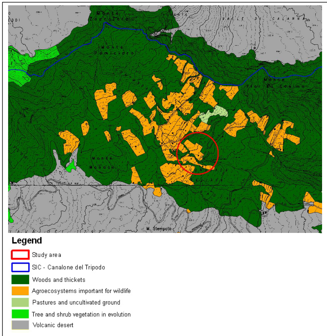
Fig. 2.6.1 Wildlife interest areas in the study area. (from draft of Regional Landscape Plan, field 13). The sampling area is shown with a red circle.
