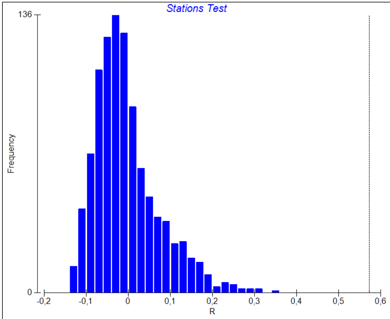
Graph. 7.1.4 – ANOSIM tests: distribution of expected frequencies of R (histogram) compared with the observed value of R ( 0,57 ) (continuous line) between the traps of the stations investigated in regards to Families of the Coleoptera.
