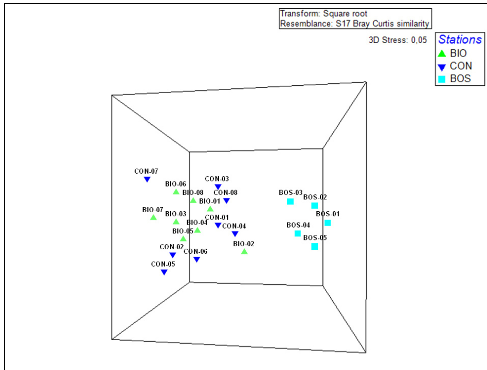
Graph. 7.1.3 – The Nonmetric Multi Dimensional Scaling (NMDS) elaborated on the Bray-Curtis similarity matrix between the traps of investigated stations in regards to Families of the Coleoptera (3 D vision).
