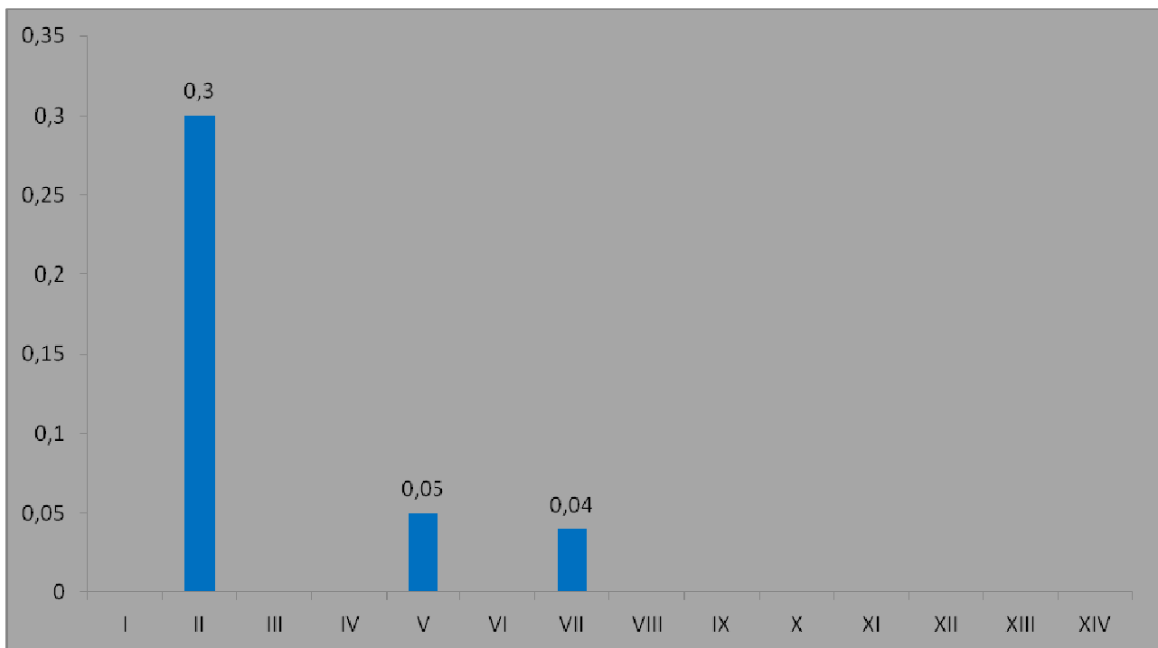
Graph. 5.3.18 - Trends in capture frequencies (CS) of Xantholinus sp. in individual sampling periods.
