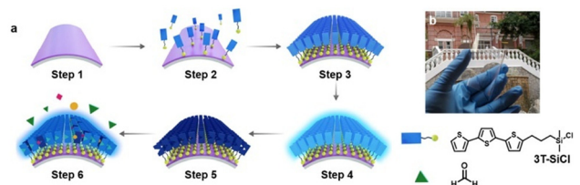
Fig. 7 (a) Schematic of the steps involved in SAM sensor development. (b) Real image of the flexible sensor. Reproduced from ref. 65 with permission from the American Chemical Society, copyright 2021.
