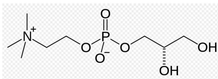
Figure A: Chemical structure of choline alfoscerate
