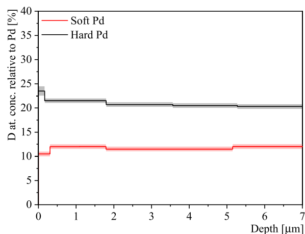
Fig. 2. Deuterium concentration relative to Palladium as a function of depth in the target, measured in soft Pd (red line) and hard Pd (black line) foils using the Nuclear Reaction Analysis technique. Shaded areas represent errors to the fitted deuterium concentrations obtained using SIMNRA code [27].
