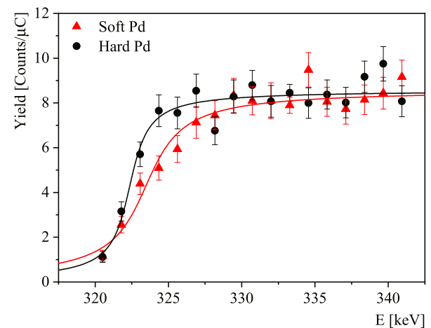
Fig. 8. \gamma -ray yields for the ^1\text{H}(^{19}\text{F},\alpha\gamma)^{16}\text{O} reaction as a function of the centre-of-mass energy, in the soft Pd (red triangles) and the hard Pd (black circles) foils near the resonance energy of 323.31 keV in the centre-of-mass system. The solid lines represent fits with Eq. (6). One can observe that above the resonance energy the measured yields are constant, confirming a uniform hydrogen distribution throughout the analysed target depth of about 70 nm.
