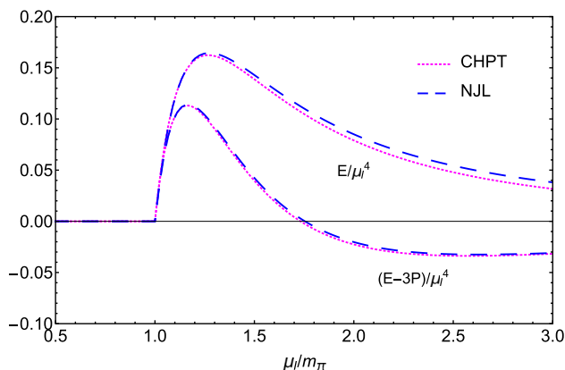
Fig. 2 The normalized energy density E/\mu_I^4 and trace anomaly (E - 3P)/\mu_I^4 as functions of \mu_I/m_\pi at zero temperature. The result from CHPT at zero temperature is also included for comparison
