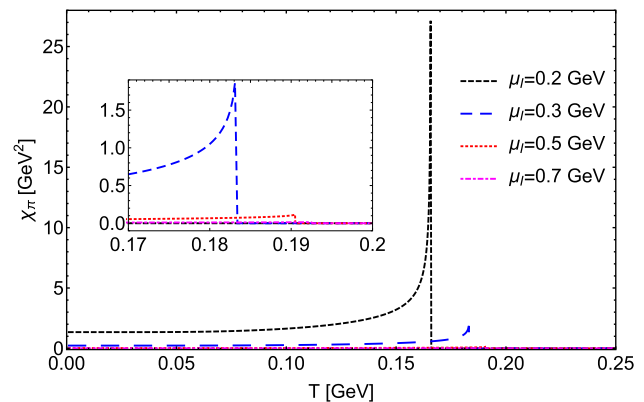
Fig. 5 The variation behaviors of the pseudoscalar susceptibility against temperature for several values of \mu_I
