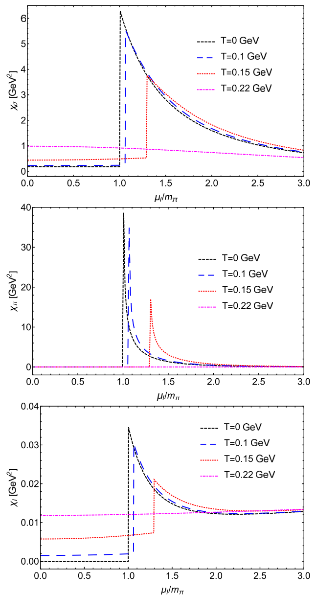
Fig. 3 The variation behaviors of chiral susceptibility \chi_\sigma , pion susceptibility \chi_\pi , and isospin number susceptibility \chi_I with respect to \mu_I/m_\pi for several values of the temperature
