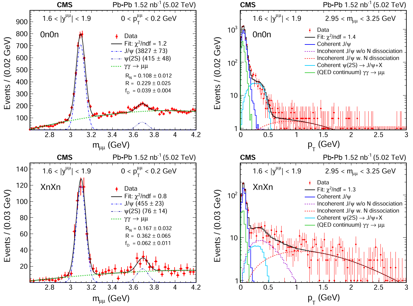
FIG. 5. The invariant mass distribution (left) of \mu^+\mu^- pairs in the dimuon p_T < 0.2 GeV range from the 0n0n (upper) and XnXn (lower) neutron classes. The results of the fit are shown by the various curves, and the corresponding values of the \chi^2 /number of degrees of freedom (ndf) and the fitted number of J/\psi and \psi(2S) candidates are given. The values of the factors R_N , R , and f_D , defined below, are also shown. The transverse momentum distribution (right) of \mu^+\mu^- pairs with a dimuon invariant mass in the J/\psi mass window of ( 2.95 < m_{\mu^+\mu^-} < 3.25 GeV) in the 0n0n (upper) and XnXn (lower) neutron classes. Again, the results of the fit are shown by the various curves. In both plots, the vertical bars on the data points represent statistical uncertainty.
