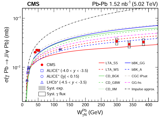
FIG. 3. The total coherent J/\psi photoproduction cross section as a function of W_{\gamma N}^{\text{Pb}} from the CMS measurement in Pb-Pb UPCs at \sqrt{s_{\text{NN}}} = 5.02 TeV. Approximated results (implied by the asterisk) from the ALICE [13,14] and LHCb [17] experiments are displayed for specific rapidity regions, where the two-way ambiguity effect is expected to be negligible. The W_{\gamma N}^{\text{Pb}} values used correspond to the center of each experiment's rapidity range. The vertical bars and the shaded and open boxes represent the statistical, experimental, and theoretical (photon flux) uncertainties, respectively. The predictions from various theoretical calculations [32,33,62–65] are shown by the curves.
