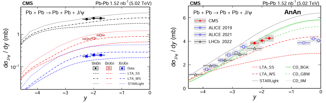
FIG. 2. The differential coherent J/\psi photoproduction cross section as a function of rapidity, in different neutron multiplicity classes: 0n0n, 0nXn, and XnXn (left); AnAn (right). The small vertical bars and shaded boxes represent the statistical and systematic uncertainties, respectively. The horizontal bars show the bin widths. Theoretical predictions from LTA weak and strong shadowing [33], color dipole models (CD_BGK, CD_BGW, and CD_IIM) [62], and STARlight [46] are shown by the curves. The right plot also displays the results from the ALICE [13,14] and LHCb [17] experiments.
