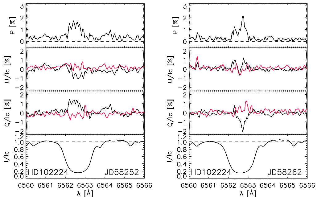
Fig. 6.9.: HD102224: linear polarisation across the H_\alpha absorption profile. An important variability within a time interval of 10 days is present.
