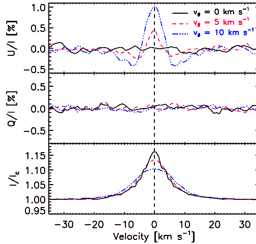
Fig. 5.23.: Polarisation of a spectral line emitted from a 30^\circ open undraptured disk seen at \cos \theta = 0.85 . The black solid line is for a non-rotating disk, the red dashed line for a disk with rotational velocity v_\theta = 5 \text{ km s}^{-1} and the blue dashed solid line for a disk with v_\theta = 10 \text{ km s}^{-1} . To justify the null Stokes Q profiles, a PA = 45^\circ has been assumed.
