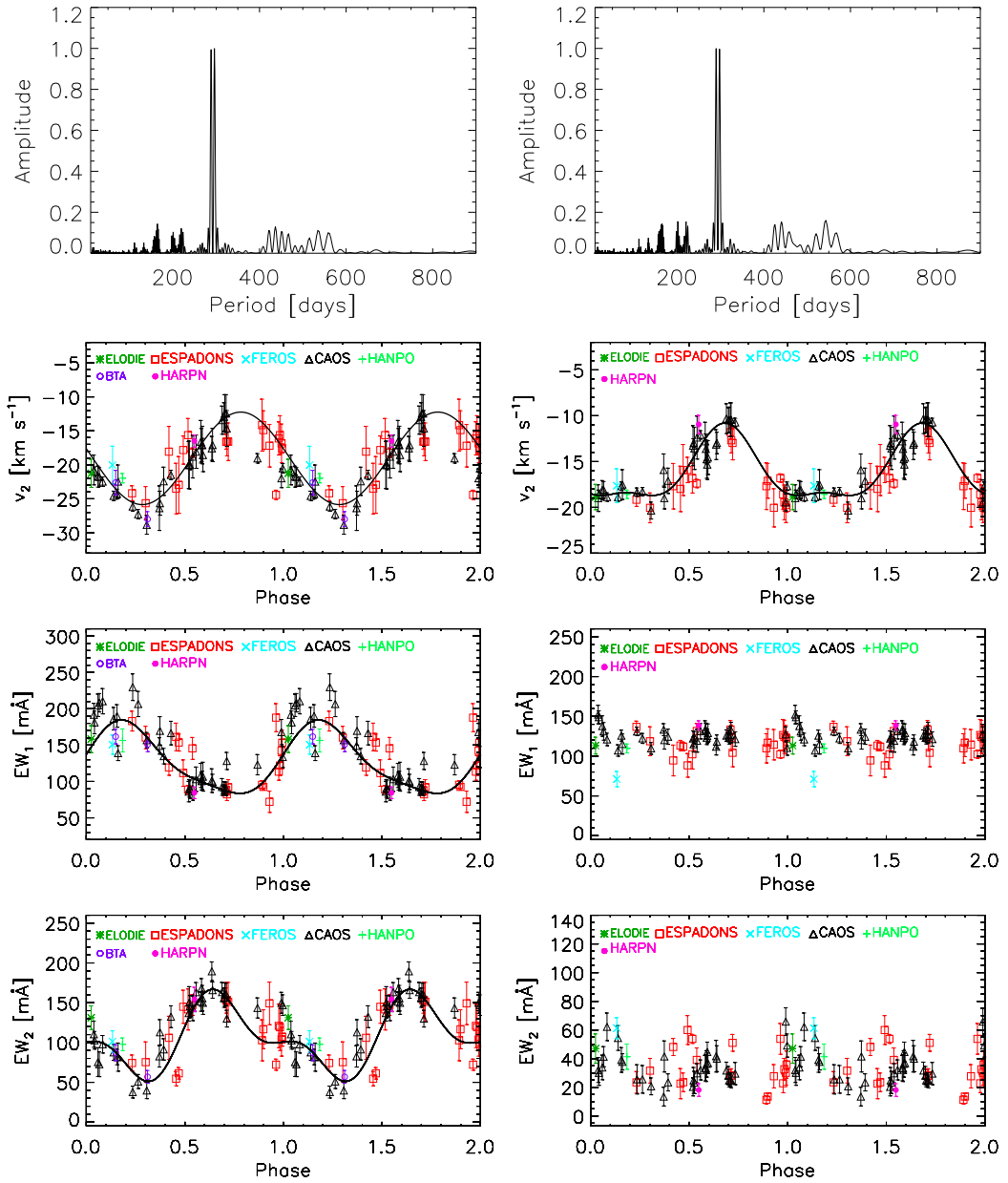
Fig. 5.34.: Gaussian Decomposition results for the BaII 6141.712 Å line (left) and YI 5087.418 Å line (right). From top to bottom: CLEANED Periodogramm of the relative velocity between the centroid of the two components of the profile, clearly showing a peak close to the orbital period; relative velocity in phase with the orbital period; equivalent widths of the central component ( EW_1 ) and of the blue-shifted component ( EW_2 ) again in phase with the orbital period.
