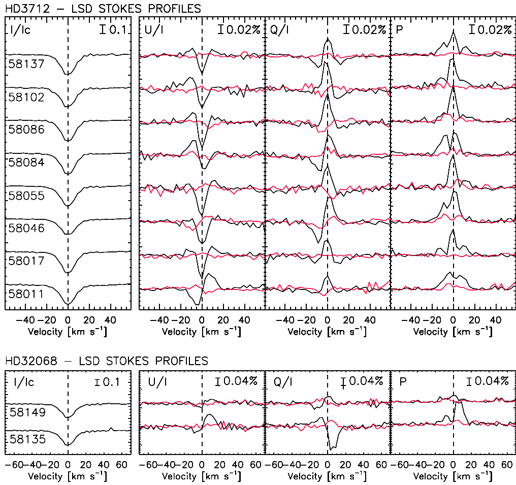
Fig. 6.7.: CAOS LSD profiles of the selected stars which show variable polarisation. Profiles were vertically shifted for clarity.
