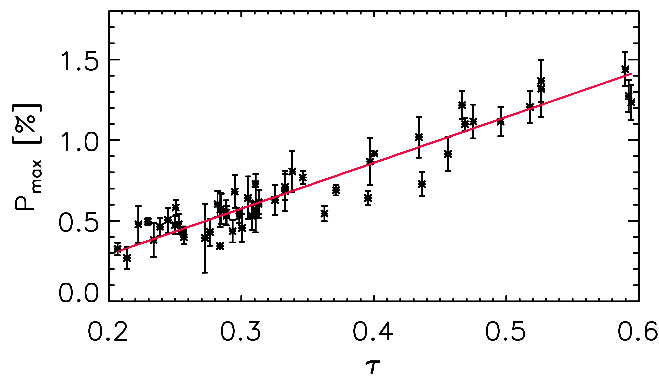
Fig. 5.9.: Top: examples of spectral lines with equal depth showing that, within errors, polarisation does not depend on wavelength. Bottom: maximum of the polarisation across spectral lines versus optical depth.
