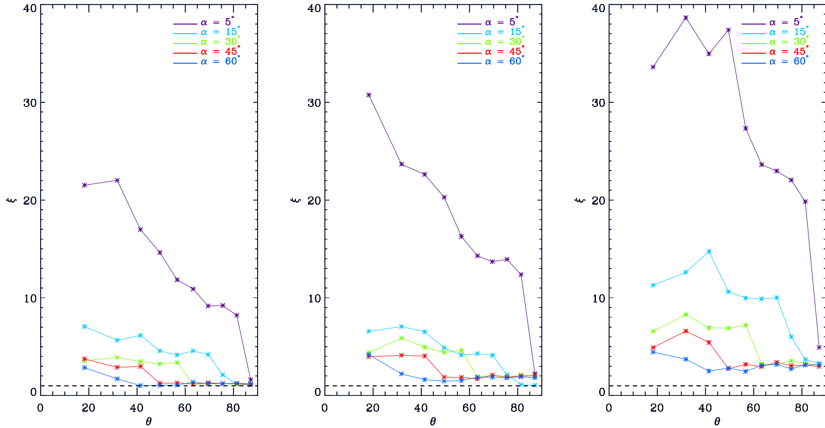
Fig. A.11.: \xi ratio between total polarisation from scattering by undisrupted disk and by disk with inner hole versus \theta view angles from different disk opening angles. Left: R_{int}/R_{ext} = 0.1 . Center: R_{int}/R_{ext} = 0.5 . Left: R_{int}/R_{ext} = 0.75 .
