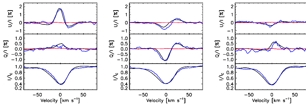
Fig. 5.10.: ESPaDOnS: Comparison between the Stokes parameters of the Fe II 4508.288 Å (black) line and LSD profiles (blue). LSD null polarization in red. From the left, spectra were acquired on HJD 53604.753, 53961.777 and 54878.132.
