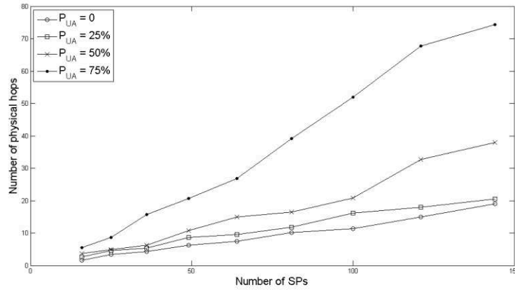
Figure 3-11: Effect of the blacklist on the number of physical hops for different percentage of unavailability. Random topology.
