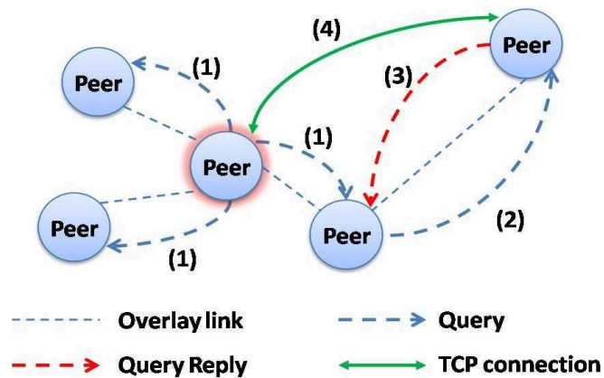
Figure 2-4: Gnutella architecture.
