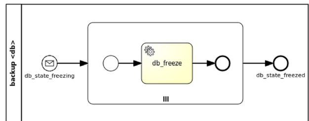
Fig. 11 Database Backup workflow for a WordPress scenario
