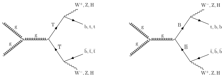
Figure 1. Representative Feynman diagrams of the pair production of T\bar{T} (left) and B\bar{B} (right), with decays to third generation quarks and SM bosons.
