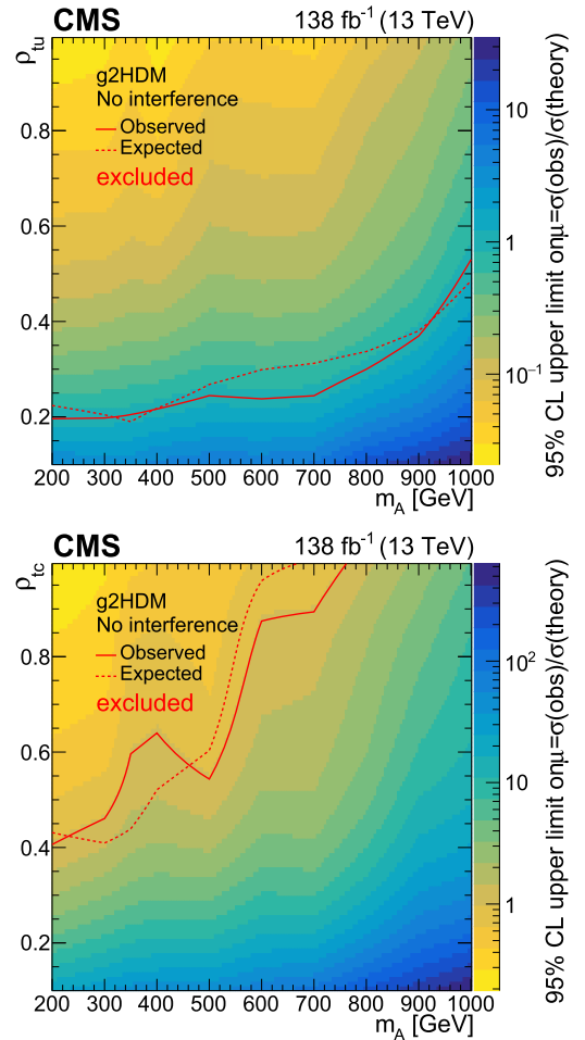
Fig. 6. Observed 95% CL upper limit on the signal strength as a function of m_A and \rho_{\text{tu}} (upper) and \rho_{\text{tc}} (lower) for g2HDM without the A-H interference, for the combination of the e^\pm e^\pm , \mu^\pm \mu^\pm , and e^\pm \mu^\pm categories. The color axis represents the observed upper limit on the signal strength. Expected (dashed lines) and observed (solid lines) exclusion contours are also shown.
