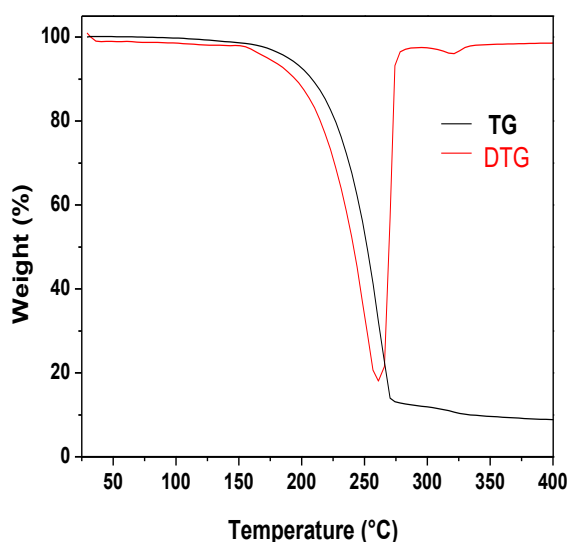
Fig 2.1.1.2 TG and DTG profiles of \text{Ba}(\text{hfa})_2 \cdot \text{tetraglyme} under \text{N}_2 flow at atmospheric pressure in the 30\text{--}400\text{ }^\circ\text{C} temperature range.
