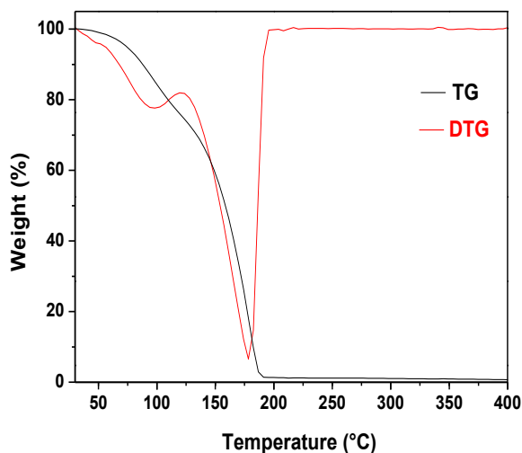
Fig. 2.1.2.2 TG and DTG profiles of Mg(hfa)_2 \cdot 2H_2O \cdot 2diglyme under N_2 flow at atmospheric pressure in the 30–400 °C temperature range.
