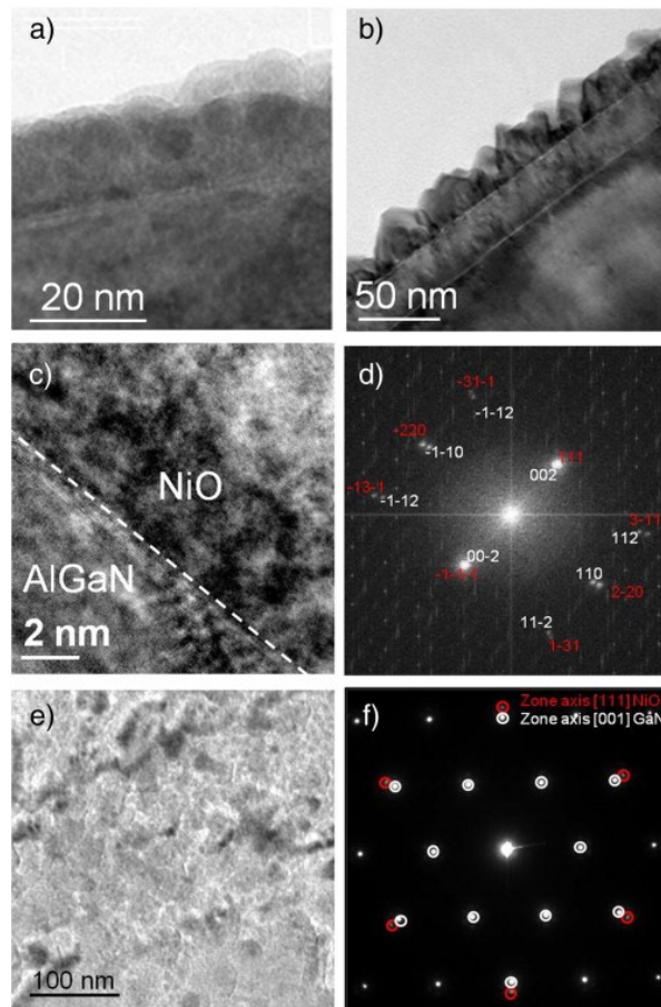
Fig. 2.2.2.3 TEM cross-sections of NiO films deposited at (a) 500 °C and (b) 750 °C. High resolution TEM image (c) of the NiO/AlGaIn interface and its relative Fast Fourier Transform image (d). TEM in-plane image (e) of the NiO film deposited at 500 °C and the relative electron diffraction patterns (f) from the substrate (white circles) and from the NiO film (red circles).
