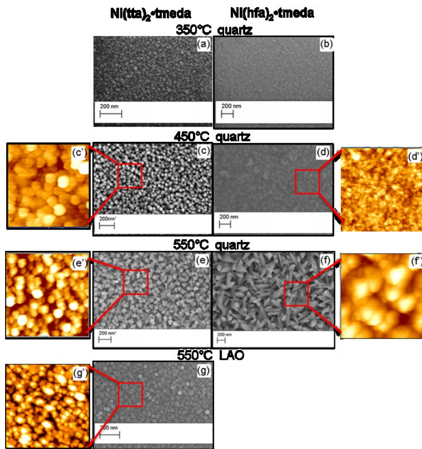
Fig. 2.2.1.7 FE-SEM images of NiO films deposited on (a-f) quartz substrate and (g) on LAO from (a, c, e, g) Ni(tta) 2 •tmeda and (b, d, f) Ni(hfa) 2 •tmeda. The corresponding 1µm x 1µm AFM topographical images (c', d', e', f' and g') are also shown.
