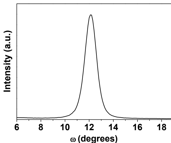
Fig. 3.2.3.3 Rocking curve of the 040 reflection of the BMF film deposited on STO (110).
