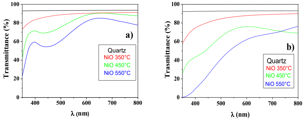
Fig. 2.2.1.9 Transmittance spectra of NiO films on quartz from (a) Ni(tta)_2 \cdot tmeda and (b) Ni(hfa)_2 \cdot tmeda as a function of temperature.
