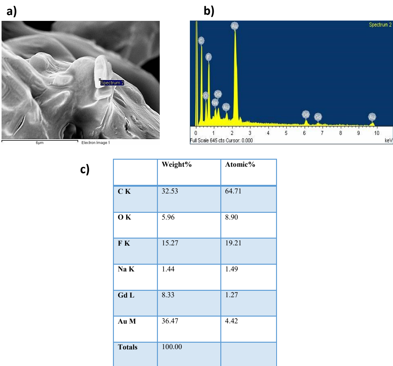
Fig. 2.3.2.1 FE-SEM image (a), EDX spectrum (b) and quantitative analysis (c) of \text{NaGd}(\text{hfa})_4 \cdot \text{tetraglyme} .
