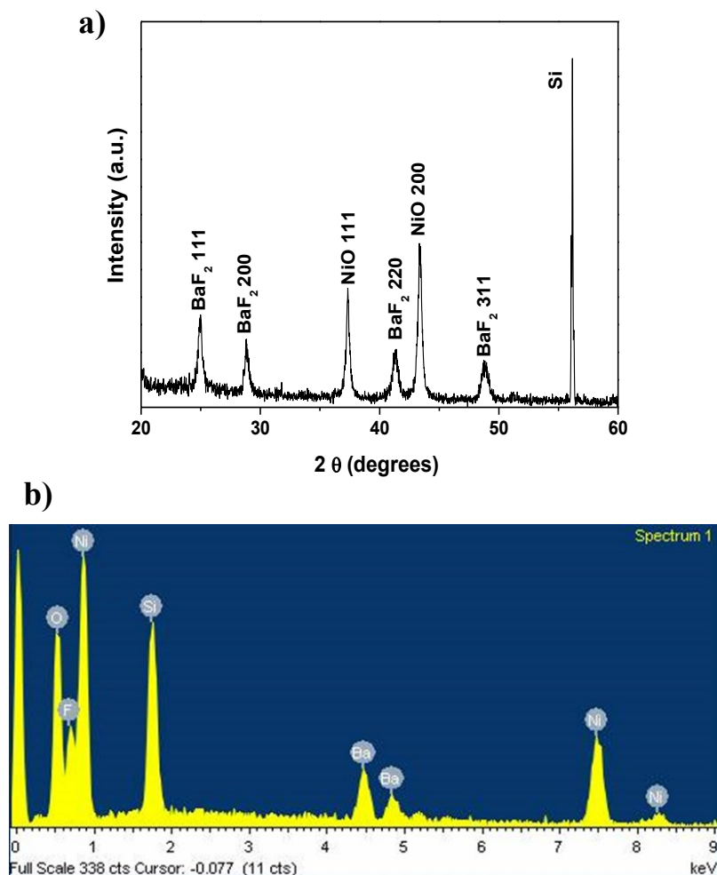
Fig. 3.1.1 XRD pattern (a) and EDX spectrum (b) of a BaNiF 4 film deposited at 600°C with oxygen flow.
