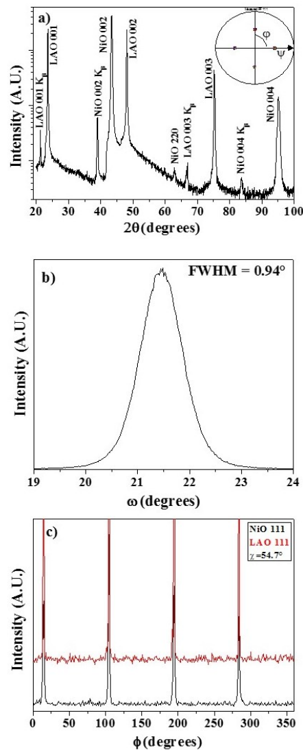
Fig. 2.2.1.5 a) XRD pattern of a film deposited on LAO (001) substrate at 550°C using the Ni(tta)_2 precursor; the inset reports the 111 pole figure ( 2\theta = 37.25^\circ ) of the NiO film; b) rocking curve of 002 reflection of the epitaxial NiO film; c) \Phi -scans using the 111 reflections as poles for the NiO and LaAlO_3 substrate.
