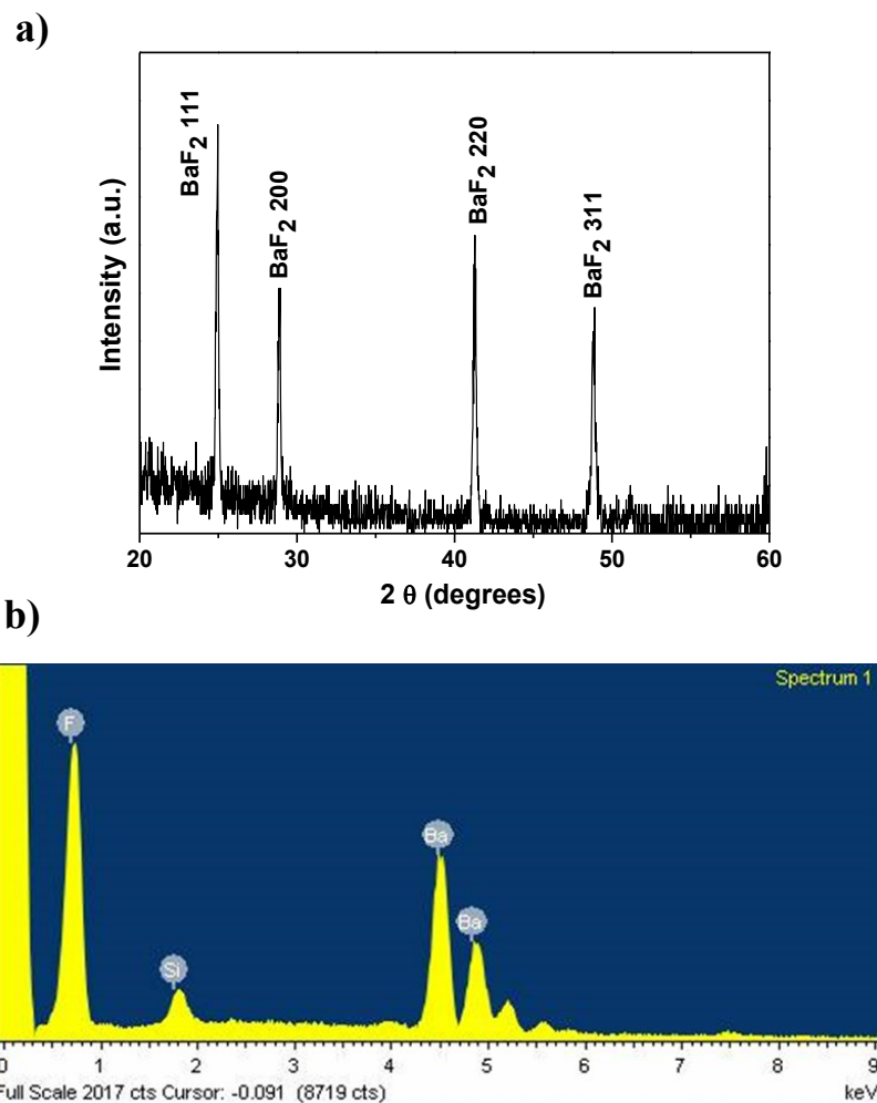
Fig. 3.1.2 XRD pattern (a) and EDX spectrum (b) of BaNiF 4 film deposited at 600°C without oxygen flow.
