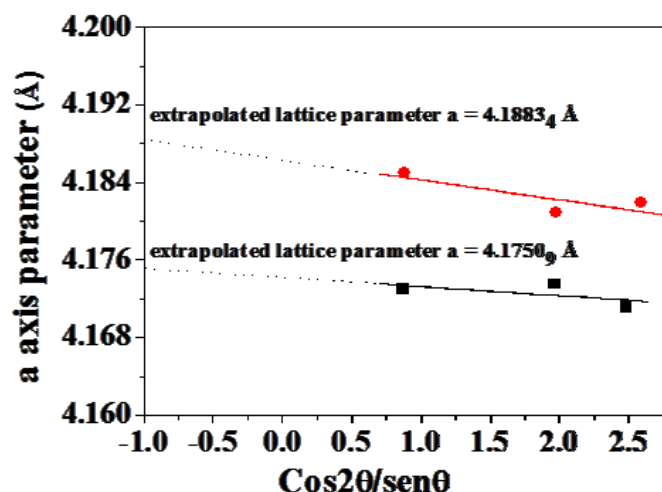
Fig. 2.2.1.4 Diagram for extrapolation of a -axis parameter of NiO phase. Red points refer to the NiO film obtained from Ni(hfa) 2 •tmeda precursor, black points refer to the NiO film obtained from Ni(tta) 2 •tmeda.
