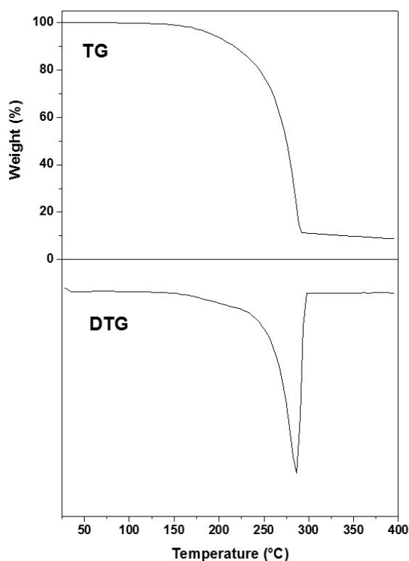
Fig 2.3.1.4 TG and DTG profiles of the [Y(hfa)_4][Na\cdot tetraglyme]^+ complex under N_2 flow at atmospheric pressure in the 25-400° °C temperature range.
