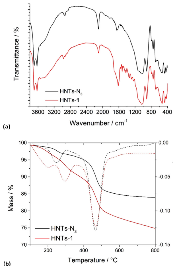
Fig. 1 (a) FT-IR spectra and (b) thermoanalytical curves (solid lines) and their derivatives (dashed lines) of HNTs- \text{N}_3 and HNTs-1 nanomaterials.
