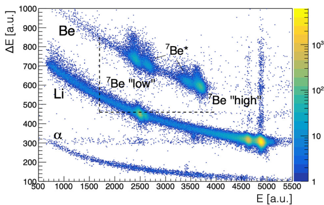
Fig. 2 \Delta E vs. E scatter plot obtained from the irradiation of a \text{CH}_2 target with a 28-MeV ^7\text{Li} beam. The bands identify nuclei of different Z ( \alpha , Li and Be), as discussed in the text. Neutrons traveling towards the TPC are produced in association with the ^7\text{Be} nuclei of the locus labeled as “ ^7\text{Be} low”. The dashed lines show the thresholds used in the normal operating conditions for the \Delta E and E detectors, and which are meant to suppress the dominant contribution from Li
