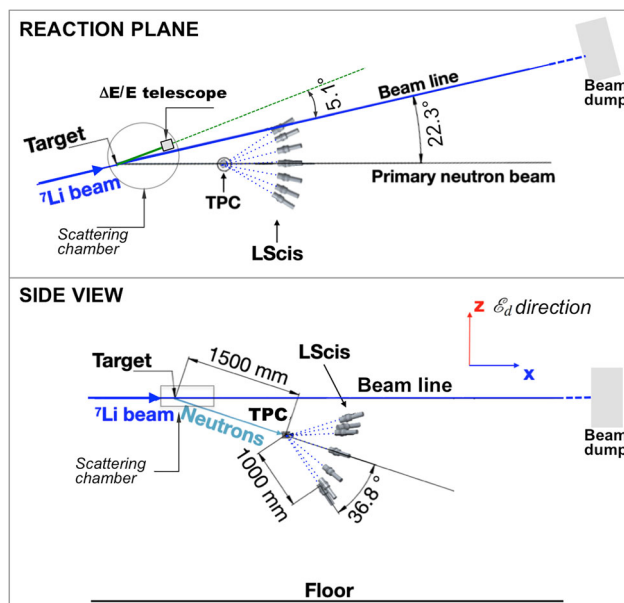
Fig. 1 Schematic layout of the ReD experimental setup (not in scale). Upper panel is the view of the p(^7\text{Li}, ^7\text{Be})n reaction plane, lower panel is the side view. The primary ^7\text{Li} beam travels along the x axis and enters the vacuum scattering chamber which hosts the \text{CH}_2 target and the \Delta E/E telescope. Neutrons emitted by the p(^7\text{Li}, ^7\text{Be})n reaction undergo elastic scattering inside the TPC and are eventually detected by one of the LScis of the neutron spectrometer, that are deployed within a cone of opening \theta_{\text{LSci}} = 36.8^\circ with respect to the target-TPC axis. See text for more details
