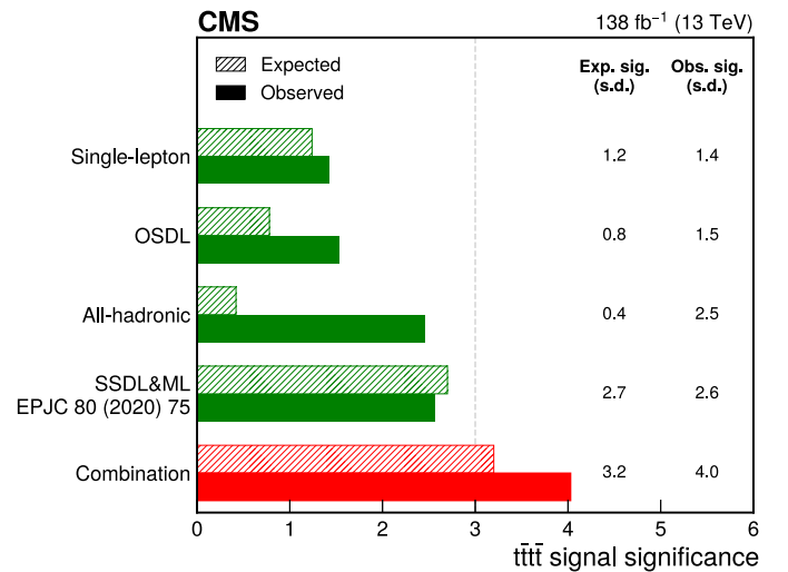
Fig. 7. Expected and observed significance (in standard deviations) for t\bar{t}t\bar{t} production from each final state and the combination with previous CMS results [21,22]. The same-sign dilepton and multilepton (SSDL&ML) final state results are from Ref. [21].
