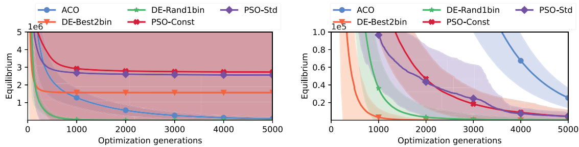
Fig. 11. Optimization of Sixteen-Member shallow truss structure using five algorithms: Left ) Convergence profile of algorithms averaged over solutions with equilibrium value of 500 and Right ) a closer snapshot of convergence profile with non-converging solutions filtered out. Algorithms ACO, DE/best/2/bin, DE/rand/1/bin, PSO-Const, and PSO-Std are in blue, orange, green, red, and purple; and they are marked with symbols \bullet , \blacktriangledown , \star , \times , \blacklozenge . The shaded width of color around a line represents the standard deviation of the convergence. The x -axis indicate number of generations and y -axis indicate objective as per Eq. (5).
