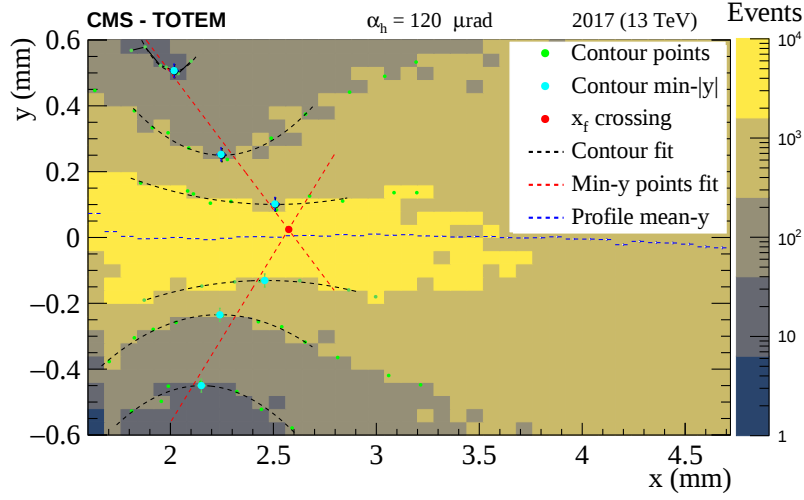
Figure 13. The (x, y) distribution of the proton impact points in the near RP detector in sector 45 for 2017 using minimum bias data, along with parabolic fits of the contours around the “pinch”. The minima of the parabolas are fitted with a straight line. The intersection of the two lines is marked with a red dot, and indicates the estimated focal point coordinate x_F . To make the contour curves and extrapolation symmetric, the mean of the histogram was aligned to 0 to remove the y offset created by the vertical dispersion \Delta y = D_y \xi . The vertical error bar on the contour minima, blue points, represents the statistical uncertainty of the fit.
