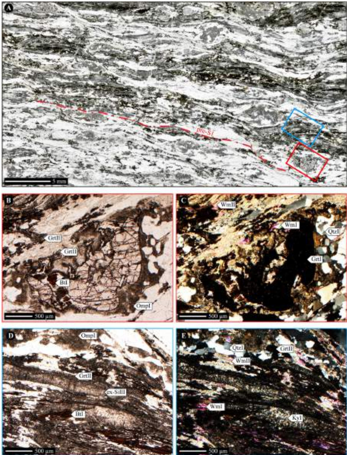
FIGURE 2 | (A) High-resolution optical scan of the entire thin section characterized by well-developed pre-S1 foliation, plane polarized light. (B) pre-alpine Grt microdomains, plane polarized light. (C) pre-alpine Grt microdomains, crossed polars. (D) pre-alpine Sill and Pl microdomains, plane polarized light. (E) pre-alpine Sill and Pl microdomains, crossed polars.
