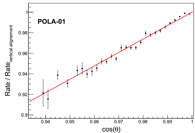
Fig. 3 Correlation between the cosmic particle rate measured by the POLA-01 detector on board of the sailboat Nanuq and its inclination with respect to the vertical. A linear fit, in red, is superimposed to the data
