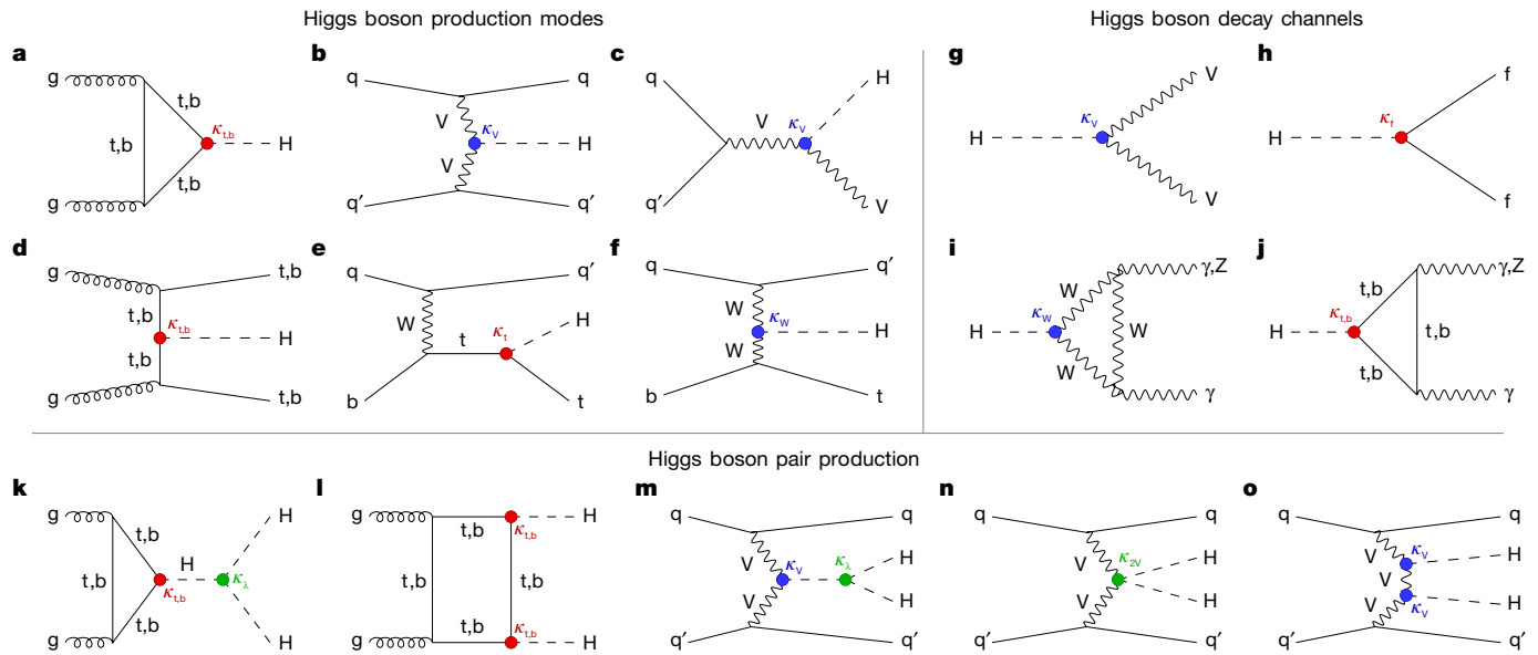
Fig. 1 | Feynman diagrams for the leading Higgs boson interactions. a–f , Higgs boson production in ggH ( a ) and VBF ( b ), associated production with a W or Z ( VH ; c ), associated production with a top or bottom quark pair ( t\bar{t}H or b\bar{b}H ; d ) and associated production with a single top quark ( tH ; e,f ). g–j , Higgs boson decays into heavy vector boson pairs ( g ), fermion–antifermion pairs ( h ) and photon pairs or Z\gamma ( i,j ). k–o , Higgs boson pair production through
