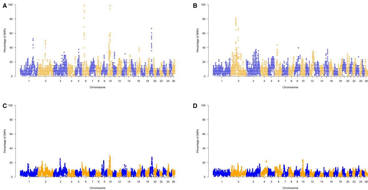
Figure 4 Manhattan plots of frequency of a single nucleotide polymorphism (SNP) in run of homozygosity islands in (A) Barbaresca, (B) Notician, (C) Sarda and (D) Valle del Belice sheep breeds.
