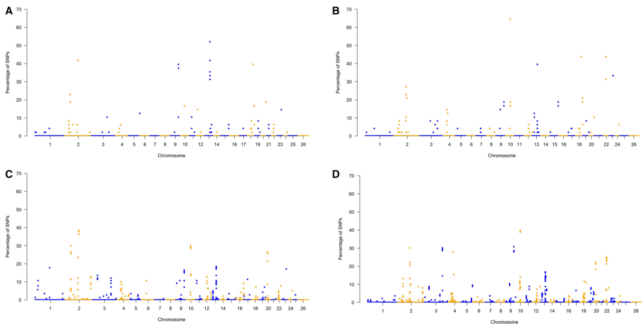
Figure 5 Manhattan plots of frequency of a single nucleotide polymorphism (SNP) in heterozygosity-rich regions in (A) Barbaresca, (B) Notician, (C) Sarda and (D) Valle del Belice sheep breeds.
