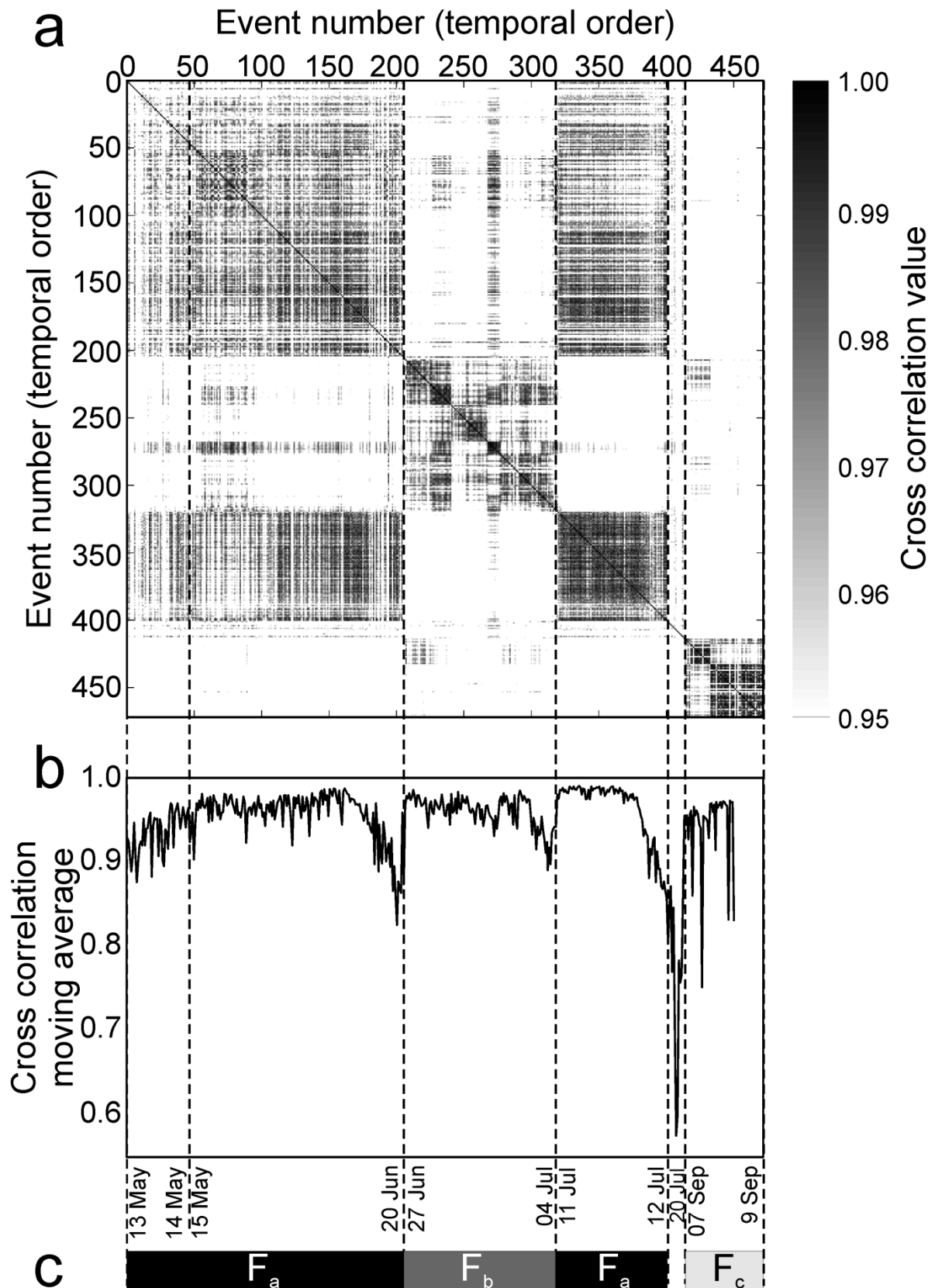
Figure 2.26: (a) Cross correlation matrix of \sim 500 infrasound events recorded at EBEL. (b) Cross correlation moving average (see text for details). (c) Black, dark grey and light grey bars indicate the occurrence periods of events belonging to F_a , F_b , F_c respectively. The dashed vertical lines show the main waveform variations.
