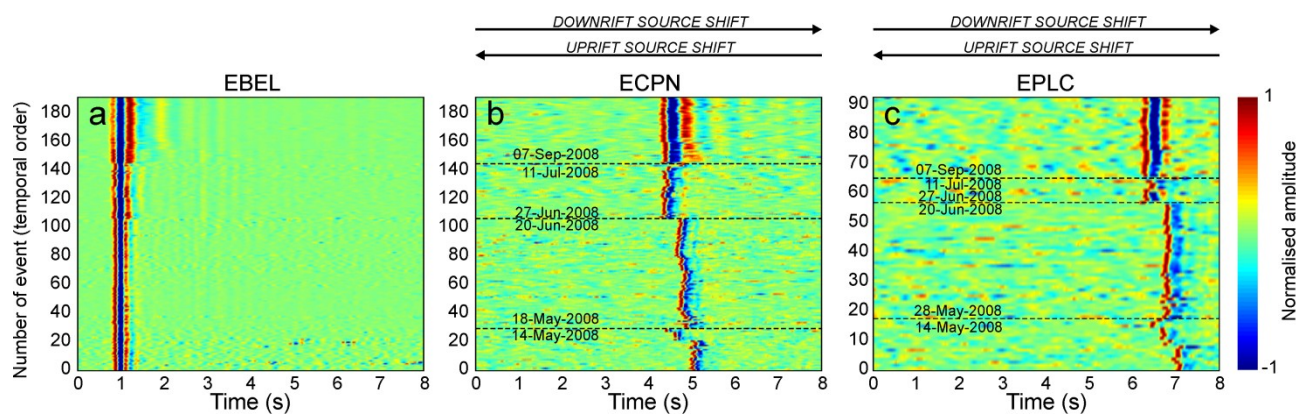
Figure 2.25: Surface plots visualizing matrixes, each of which is composed of the waveforms of the infrasound events of each station (each row is a waveform). In the x-axis the time elapsed from the onset to the end of the waveforms is reported, the y-axis represents the event number in temporal order. The amplitude of the signal is visualized with the color scale. See text for details.
