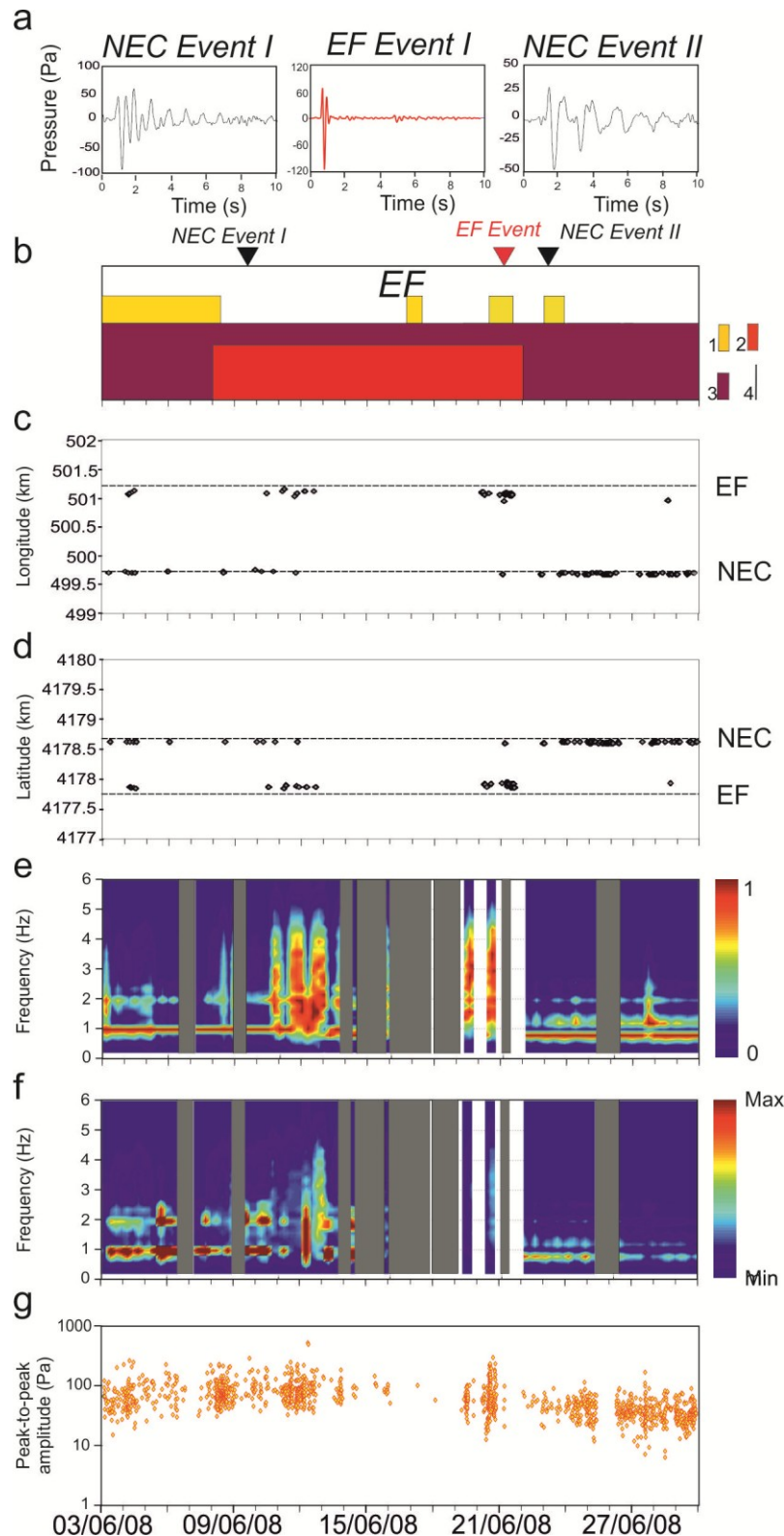
Figure 2.15: (a) Waveforms of two NEC infrasound events and an EF infrasound event recorded by EBEL station during period III (3 June – 29 June 2008). (b) Sketch of the volcanic activity of Mt. Etna at EF during period III(1: ash emission; 2: Strombolian activity; 3: effusive activity; 4: fire fountain). (c) Longitude and (d) latitude of infrasound events located during the third period. (e) Normalised pseudospectrogram, (f) pseudospectrogram (g) peak-to-peak amplitude of the infrasound events occurring at Mt. Etna during period III and recorded by EBEL station. Other symbols as in Figure 2.13.
