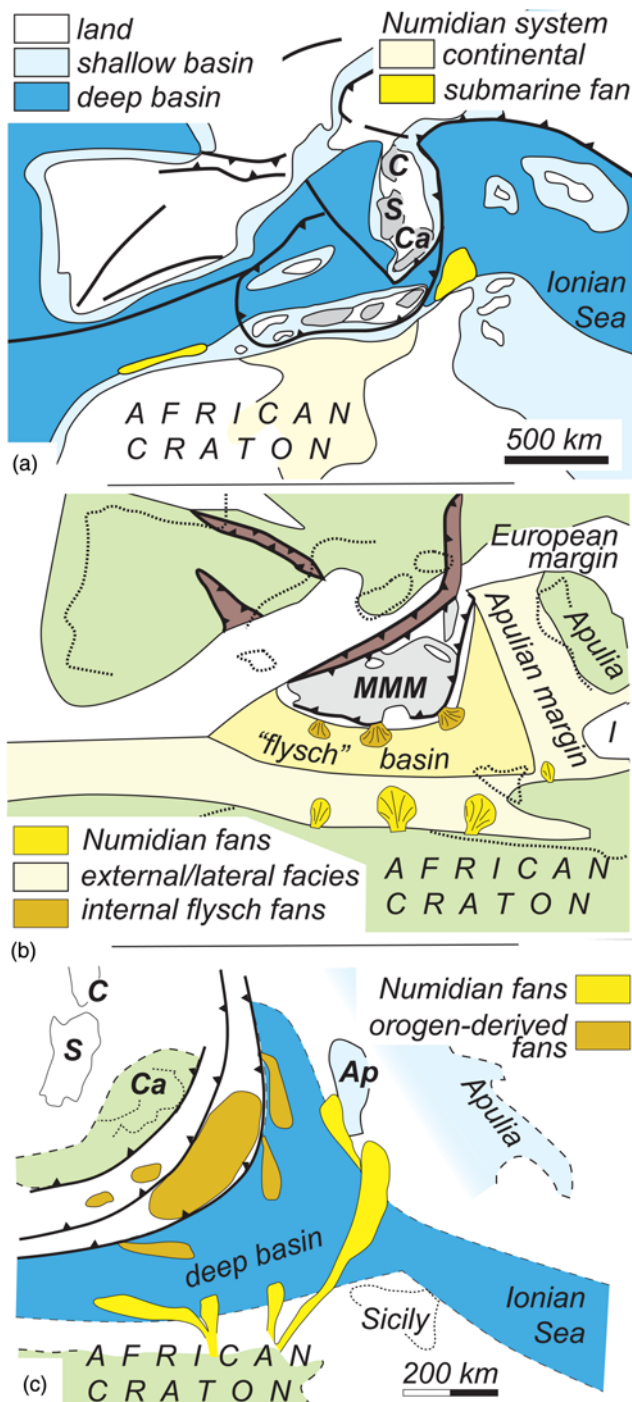
Fig. 2. A compilation of palaeogeographical models for the early Miocene in the central Mediterranean. (a) Depiction of the Numidian in Burdigalian times, forming a single unconfined fan opening into a large seaway (from Thomas et al. (2010), modified after Meulenkamp and Sissingh (2003)). (b) Representation of the Numidian and associated turbidite systems in the early Miocene, fed by fans that are significantly smaller than the size of the composite basin (from Guerrero et al. (2012)). It should be noted that the fans shown crossing Sicily (and to its east) are incompatible with the geological record (no source area, as discussed in text), and this is corrected by the model of Critelli et al. (2017); (c). (c) Critelli et al. showed the Numidian system for the Langhian forming a narrow depositional tract, ahead of the active orogenic front, and sourced from the African margin to the SW of modern Sicily. C, Corsica; S, Sardinia; Ca, Calabria; Ap, Apennine platform; I, Ionian Sea; MMM, 'Meso-Mediterranean microplate'.
