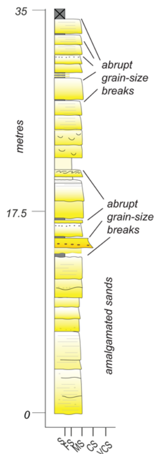
Fig. 12. Representative log of stacked bed-set in the Numidian at east of Colobraro village, Valsinni (UTM coordinates 621273.00 m E, 4449771.00 m N). Key as in Figure 8.
