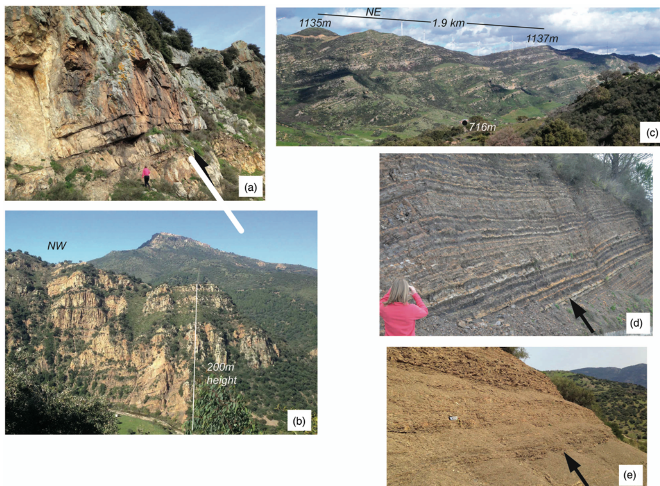
Fig. 7. Numidian outcrops in Sicily. (a) illustrates the amalgamated nature of the thicker sandstone units, near Mistretta, northern Sicily. (b) The Pollina section (see Pinter et al. 2016). (c) Monte Salici, central Sicily (see Pinter et al. 2018). (a–c) show strata interpreted to typify the main sand fairways for the Numidian turbidites. (d) Thin-bedded sandstones and siltstones, representative of off-fairway deposition, inferred to lie on the flanks of the main conduits for causative turbidity currents. These outcrops lie c 5 km lateral (SSW of) the Pollina section (b). (e) Brown siltstones and fine sandstones, again lateral to (b) and (d). (See Pinter et al. (2016) for further details.)
