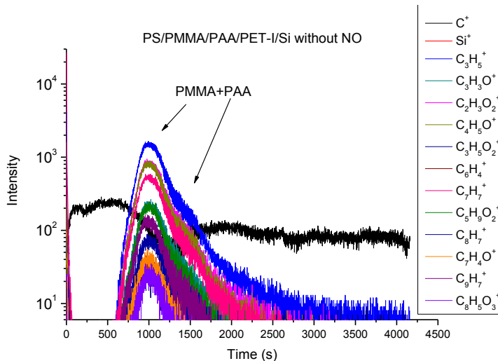
Fig. 24 - C_{60} depth profile of the PS/PMMA/PAA/PETi/Si multilayer, without NO
