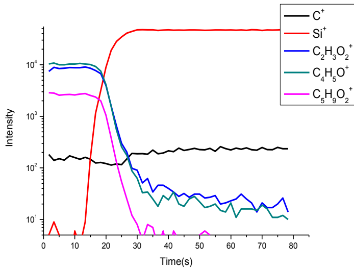
Fig. 15 – C_{60} depth profile of PMMA with NO 1.5 \times 10^{-5} mbar.
