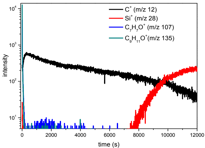
Fig. 38 - C 60 Depth profiling of PC in absence of NO dosing
