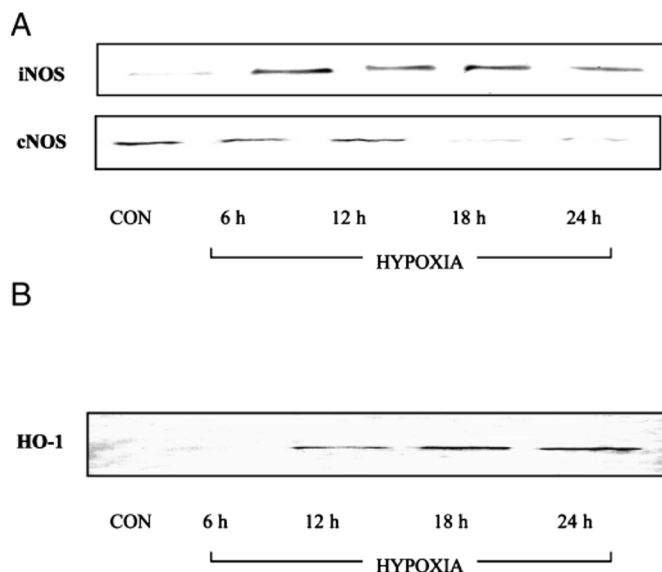
FIG. 2. Time course of endothelial iNOS, ecNOS, and HO-1 protein expression during hypoxia. Western blot analysis of cells exposed to hypoxia for different times using specific antibodies for iNOS and ecNOS (panel A) and HO-1 (panel B) is shown. Samples were processed as described under "Experimental Procedures." Each blot is representative of three independent experiments.
