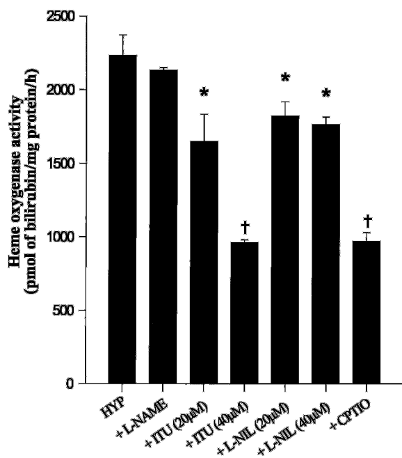
FIG. 3. Effect of ecNOS/iNOS inhibitors and the NO scavenger carboxy-PTIO on hypoxia-stimulated increase in heme oxygenase activity. Endothelial cells were exposed to hypoxia for 18 h in the presence of 1 mM L-NAME, 20 and 40 \mu M ITU, 20 and 40 \mu M L-NIL, or 100 \mu M CPTIO. Heme oxygenase activity was measured and compared with cells exposed to hypoxia for 18 h in the presence of medium alone (HYP). Each bar represents the mean ( \pm S.E.) of five or six experiments performed independently. * p < 0.05 versus HYP; † p < 0.01 versus HYP.
