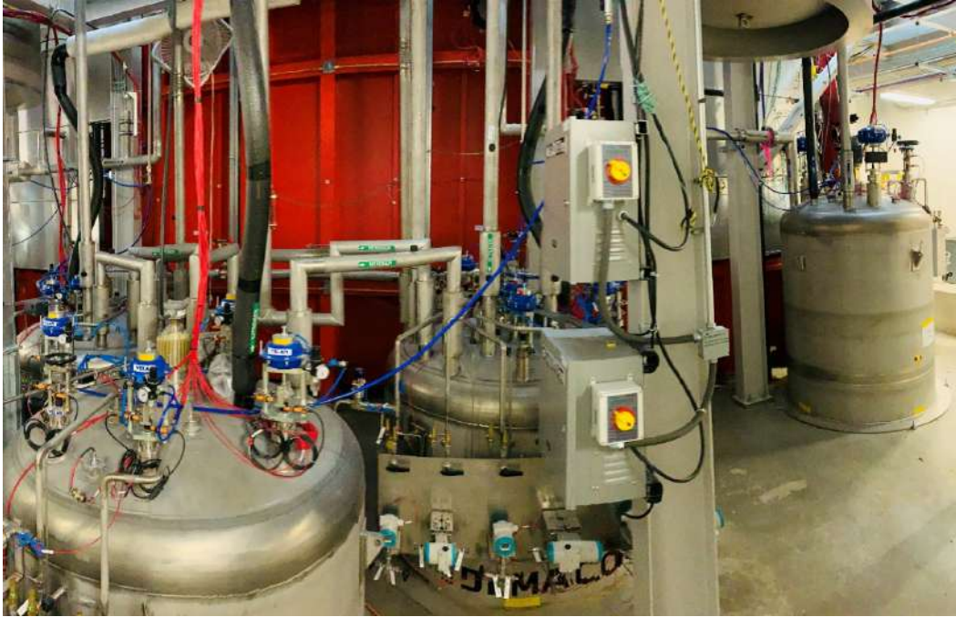
Figure 12. Three LN 2 pump boxes (left) and West LAr pump box (right).
