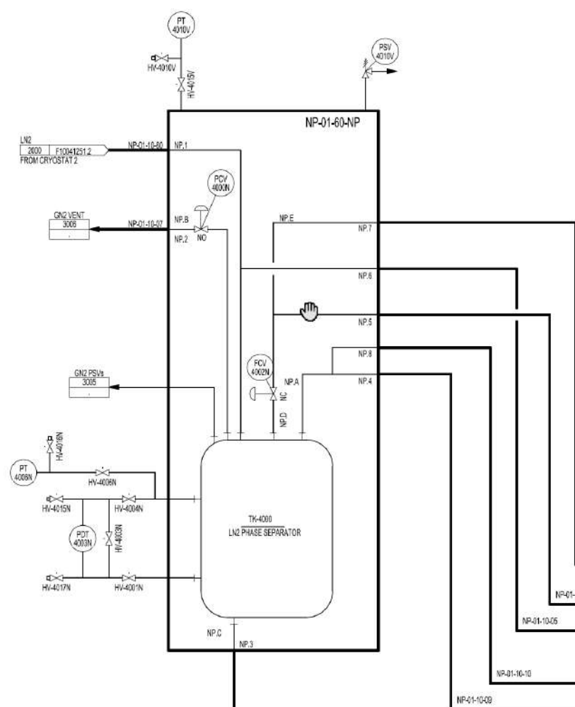
Figure 9. LN 2 phase separator box.
