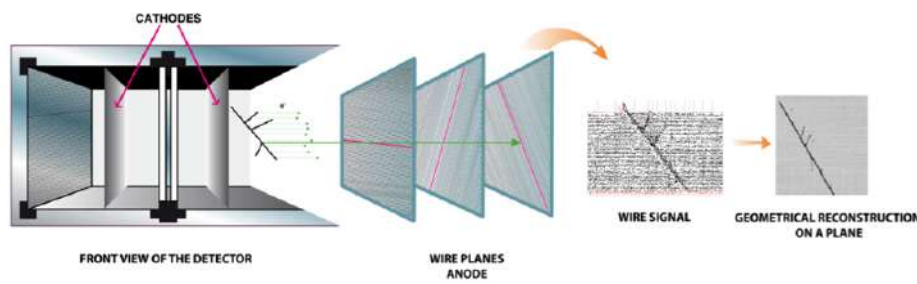
Figure 1. Sketch of the detector layout showing the LAr-TPC working mechanism.
