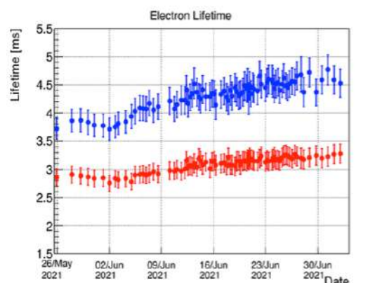
Figure 67. Free-electron lifetime during the first neutrino run (RUN0). Blue: East module; red: West module.
