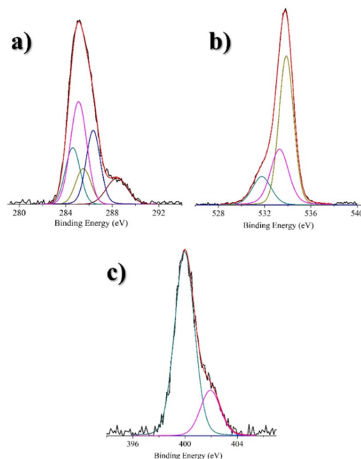
Fig. 2 In the three spectra, the blue line represents the background, and the red line superimposed to the experimental black profile refers to the sum of the Gaussian components. (a) Al \text{K}\alpha excited XPS of CNPs-DA in the C 1s binding energy region: the dark cyan, magenta, dark yellow, navy, and wine lines refer to the 284.6, 285.0, 285.5, 286.4, and 288.4 eV Gaussian components, respectively. (b) Al \text{K}\alpha excited XPS of CNPs-DA in the O 1s binding energy region: the dark cyan, magenta, and dark yellow lines refer to the 531.8, 533.3 and 533.9 eV Gaussian components, respectively. (c) Al \text{K}\alpha excited XPS of the CNPs-DA in the N 1s binding energy region: the dark cyan, and magenta lines refer to the 400.0, and 401.9 eV Gaussian components, respectively.
