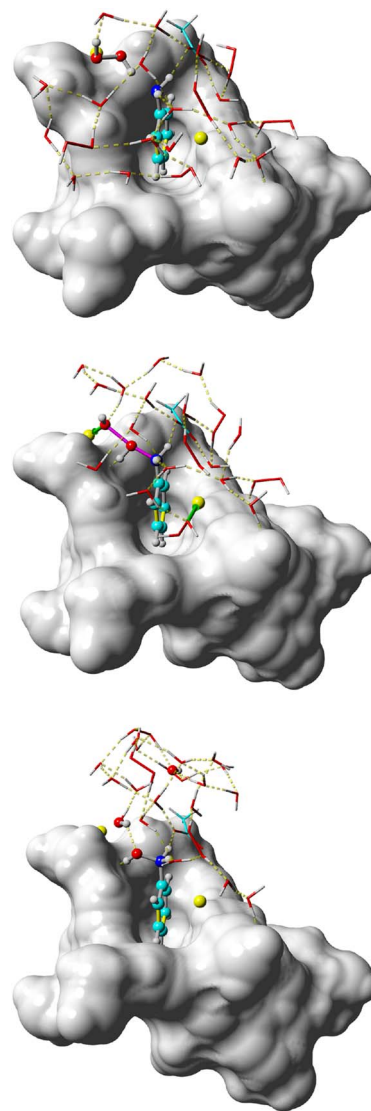
Fig. 6 Detail of 2a@PrS[6]^{COONa} (top), 2a@PrS[6]^{COONa} -TS (middle) and 2a@PrS[6]^{COONa} -P (down). Compound 2a , one interacting H 2 O 2 molecule, and Na + ions are represented as balls, H 2 O and H 2 O 2 molecules as stick lines, and PrS[6] COO- is rendered as a molecular surface. Dashed lines represent hydrogen bonds.
