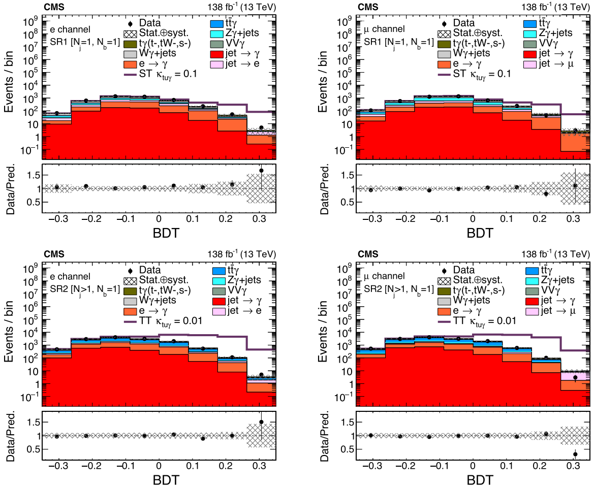
FIG. 4. The BDT output distributions for the data, the background predictions, and the expected t\gamma signal for electron (left) and muon (right) channels in SR1 (upper) and SR2 (lower). The signal distribution is normalized to a cross section corresponding to \kappa_{t\gamma} = 0.10 (0.01) for ST (TT) and is stacked on the background expectations. The first bins include underflows, and the last bins include overflows. The vertical bars on the points depict the data statistical uncertainties and the hatched bands show the combined statistical and systematic uncertainties in the estimated background processes.
