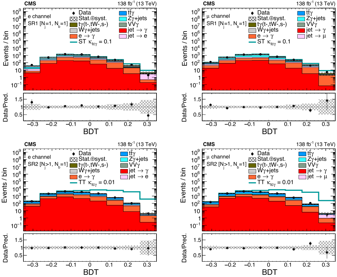
FIG. 5. The BDT output distributions for the data, the background predictions, and the expected tc\gamma signal for electron (left) and muon (right) channels in SR1 (upper) and SR2 (lower). The signal distribution is normalized to a cross section corresponding to \kappa_{tc\gamma} = 0.10 (0.01) for ST (TT) and is stacked on the background expectations. The first bins include underflows, and the last bins include overflows. The vertical bars on the points depict the data statistical uncertainties and the hatched bands show the combined statistical and systematic uncertainties in the estimated background processes.
