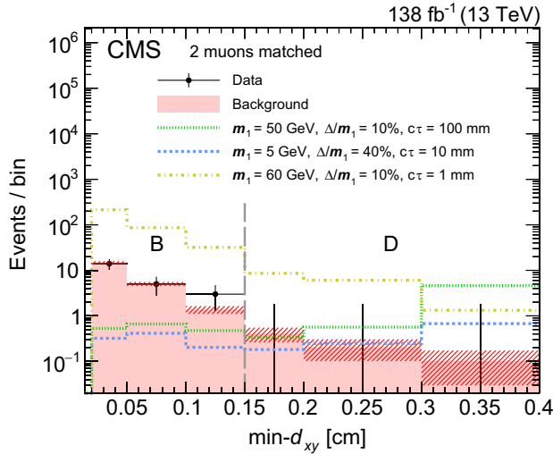
FIG. 3. Measured \min-d_{xy} distribution in the two-match category, after requiring the \min-d_{xy} muon to pass the isolation requirement I_{PF}^{\text{el}} < 0.25 (i.e., the B and D bins of the ABCD plane). Overlaid with a red histogram is the background predicted from the region of the ABCD plane failing the same requirement (the A and C bins), as well as three signal benchmark hypotheses (as defined in the legends), assuming \alpha_D is equal to the electromagnetic (EM) fine-structure constant \alpha_{EM} . The red hatched bands correspond to the background prediction uncertainty. The last bin includes the overflow.
