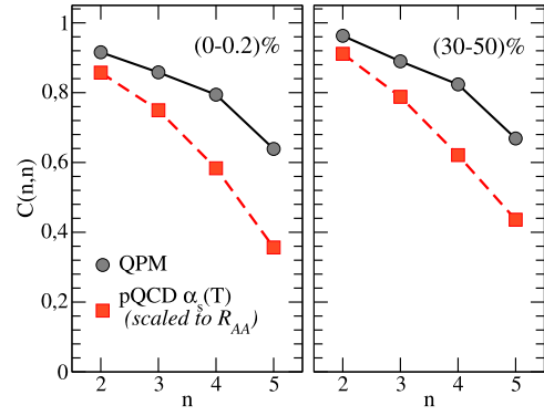
Fig. 5. Event-by-event correlation coefficient between D-meson v_n and light hadron v_n as a function of the order of the harmonic n obtained within QPM (black solid line) and pQCD (red dashed line).
