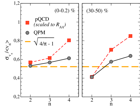
Fig. 6. \sigma_{v_n}/\langle v_n \rangle as a function of the order of harmonics n for QPM (black solid line) and pQCD (red dashed line). The orange dashed lines indicate the value \sqrt{4/\pi - 1} expected for a 2D Gaussian distribution.
