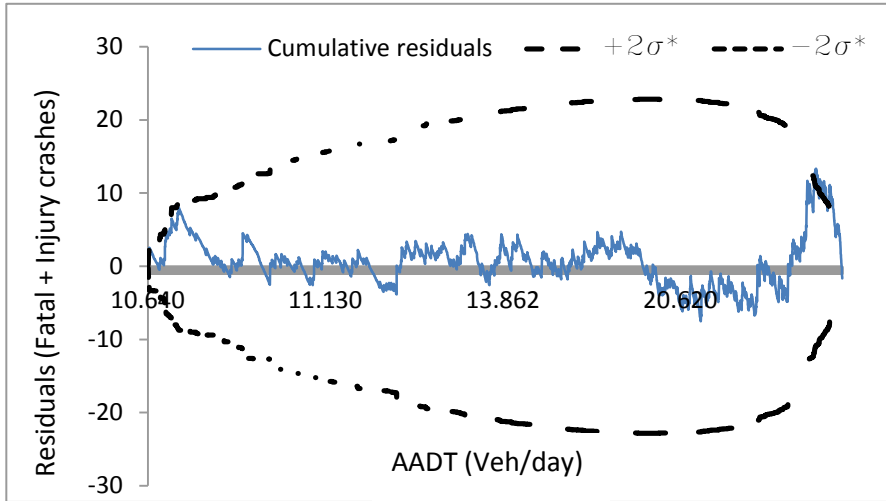
Figure 2.3. CURE Plots with \pm 2\sigma for GEE model with trend Multivariable (3)
