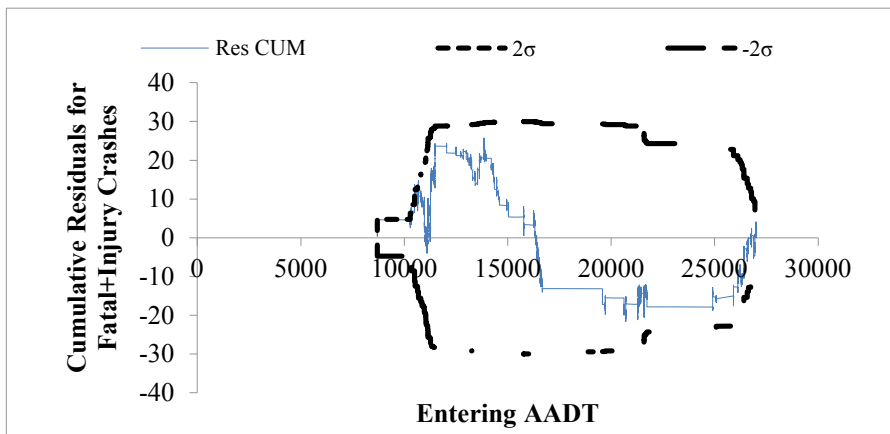
Figure 3.16. CURE Plots with \pm 2\sigma for model form C for segmentation 5.
