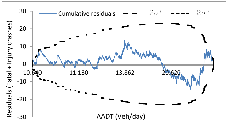
Figure 2.2. CURE Plots with \pm 2\sigma for GLM model Monovariable (2)
