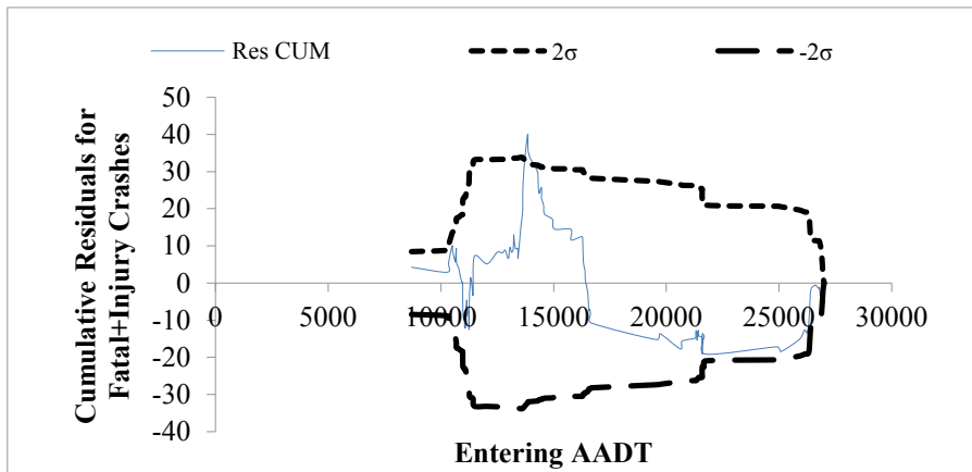
Figure 3.14. CURE Plots with \pm 2\sigma for model form C for segmentation 3.
