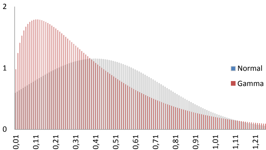
Figure 6.4. Comparison between the Gamma distribution obtained by using the values of mean and variance from the simulation and the frequency analysis of the data considering a normal distribution.
