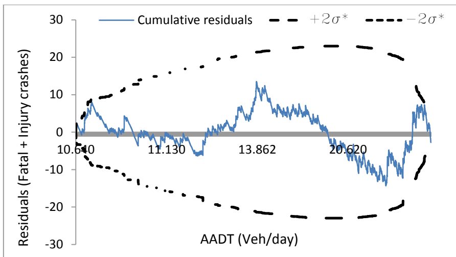
Figure 2.6. CURE Plots with \pm 2\sigma for GEE model without trend Monovariate (6)
