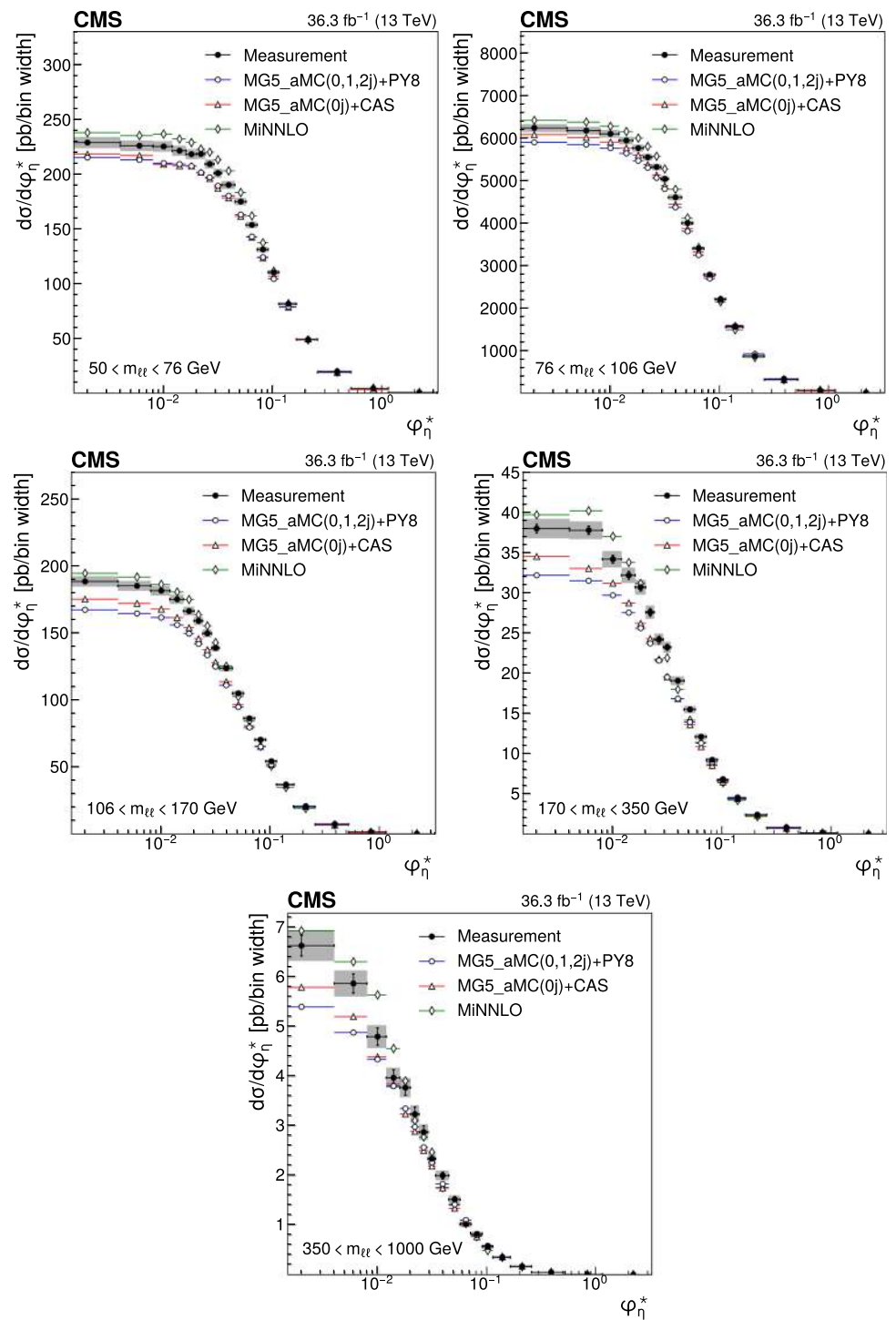
Fig. 19 Differential cross sections in \varphi_{\eta}^*(\ell\ell) in various invariant mass ranges: 50 < m_{\ell\ell} < 76 GeV (upper left), 76 < m_{\ell\ell} < 106 GeV (upper right), 106 < m_{\ell\ell} < 170 GeV (middle left), 170 < m_{\ell\ell} < 350 GeV (middle right), and 350 < m_{\ell\ell} < 1000 GeV (lower). The measurement is compared with MG5_aMC (0, 1, and 2 jets at NLO) + PYTHIA 8 (blue dots), MiNNLO PS (green diamonds) and MG5_aMC (0 jet at NLO) + PB (CASCADE) (red triangles). Details on the presentation of the results are given in Fig. 5 caption
