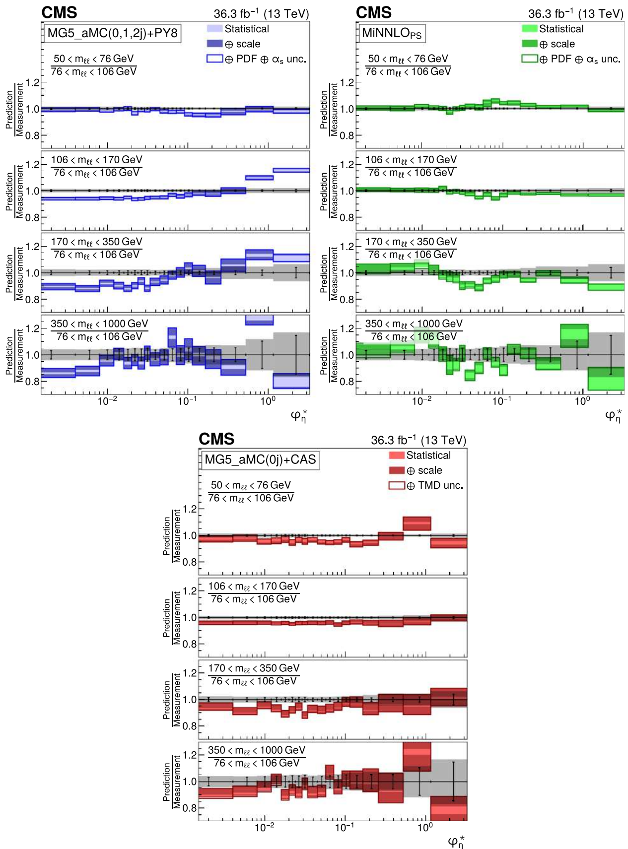
Fig. 23 Ratios of differential cross sections in \phi_{\eta}^*(\ell\ell) for invariant m_{\ell\ell} with respect to the peak region 76 < m_{\ell\ell} < 106 GeV. Compared to model predictions from MG5_aMC (0, 1, and 2 jets at NLO) + PYTHIA
