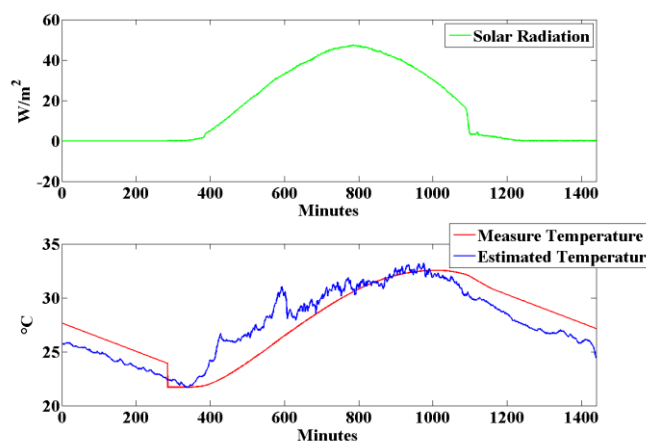
Figure 4.21: Derivation of temperature profile from radiation.
