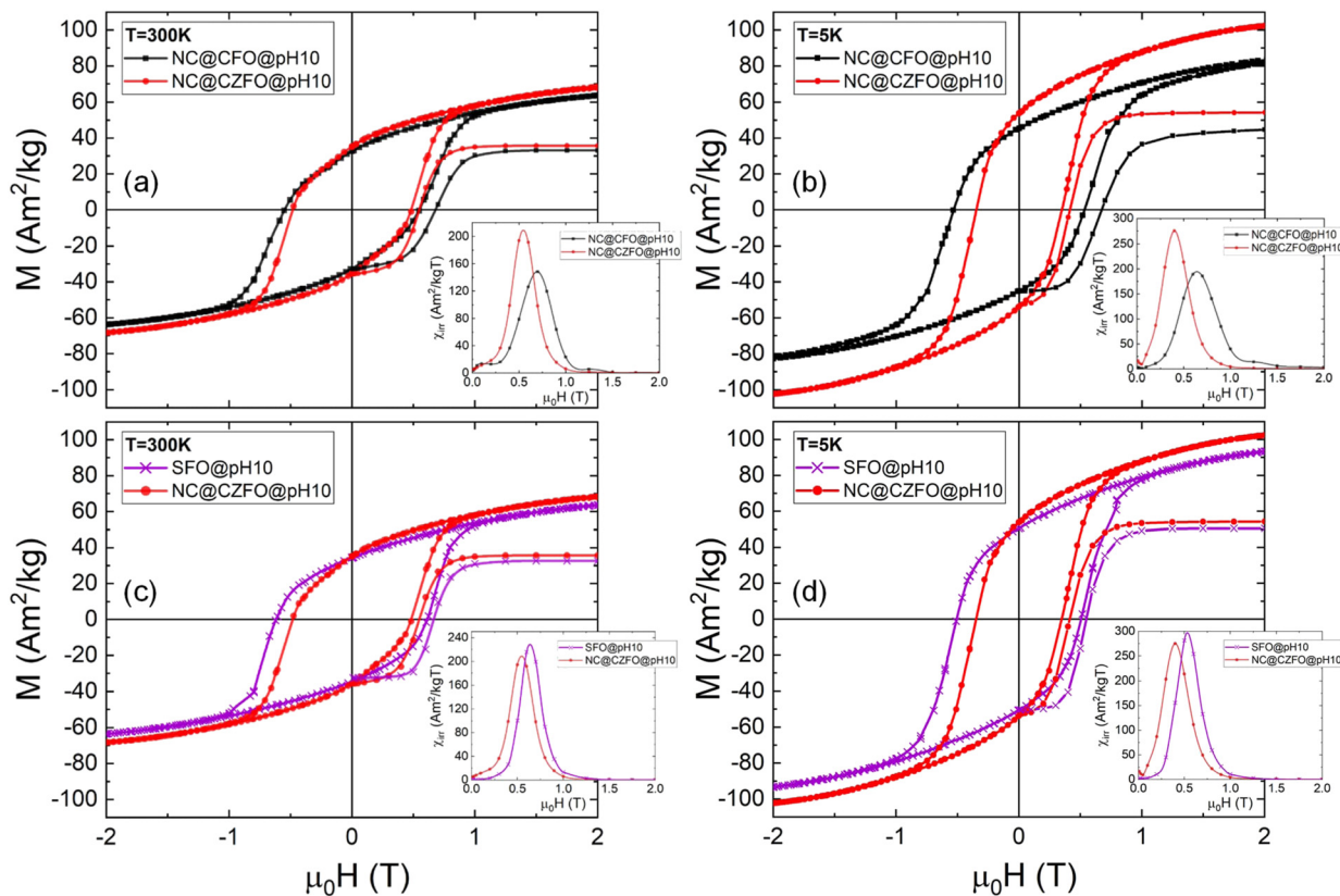
Fig. 7 Magnetization M vs. magnetic field \mu_0H curves for nanocomposites with preformed CFO and CZFO NPs at pH = 10 (NC@CFO@pH10 and NC@CZFO@pH10) and magnetization M_{DCD} vs. reverse magnetic field H curves for the corresponding samples at (a) 300 K and (b) 5 K. For comparison, panels for SFO synthesized at pH = 10 (SFO@pH10), and NC@CZFO@pH10 are reported at (c) 300 K and (d) 5 K.
