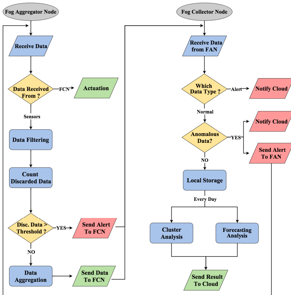
Figure 11 - Flow diagram which describes the Fog logic
