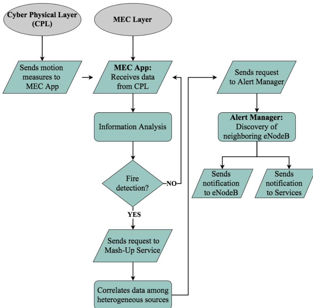
Figure 21 Flow diagram, describing the MEC logic
