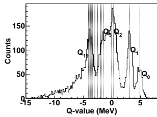
Fig. 2. Q -value spectrum of the ^{16}\text{O}(^{20}\text{Ne}, \alpha\alpha)^{28}\text{Si} channel. The dotted lines corresponds to the excited states of ^{28}\text{Si} .
