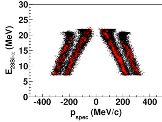
Fig. 3. ^{28}\text{Si} - \alpha relative energy vs. spectator's momentum of Monte Carlo simulation (black) and the experimental data (red).
