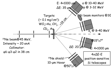
Fig. 1. Schematic view of the experimental setup.
