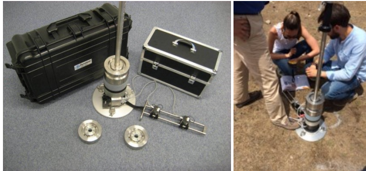
Figure 14 - LWD Dynatest 3031. University of Catania.
