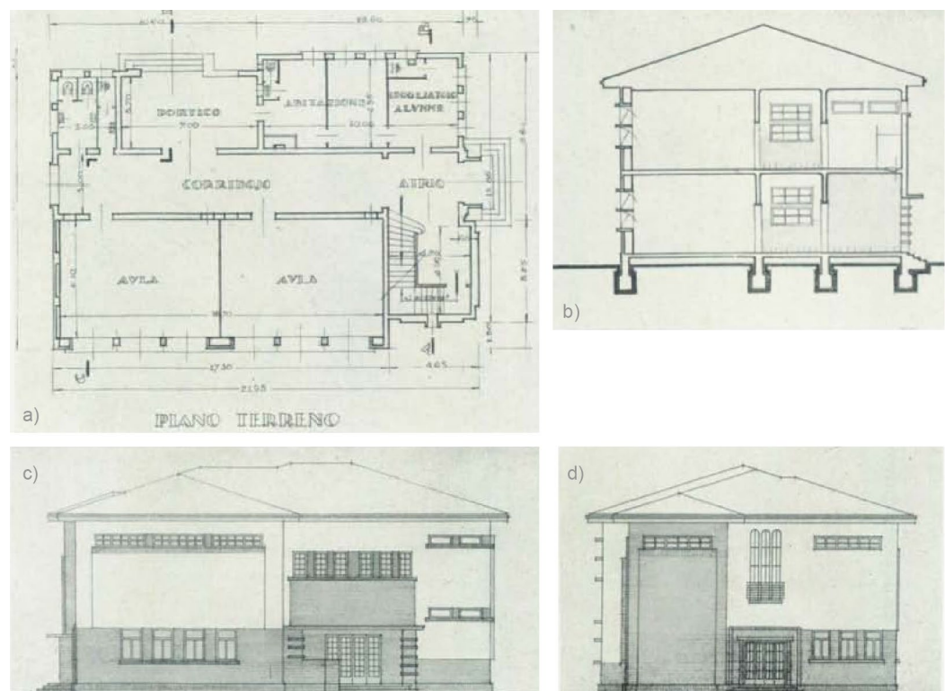
Fig. 1. Alberto Legnani, project for the agricultural training school in Castelfranco Emilia, Modena: project drawings from Domus magazine, no. 47, year IV, 1931, pp. 44-46: a) ground floor plan; b) cross section; c, d) elevations.
