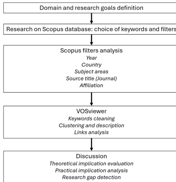
Fig. 1. Followed methodology
