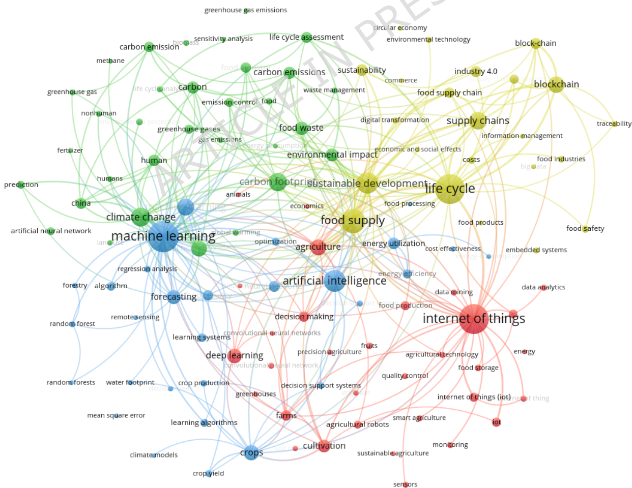
Fig. 9. VOSviewer Clustering
